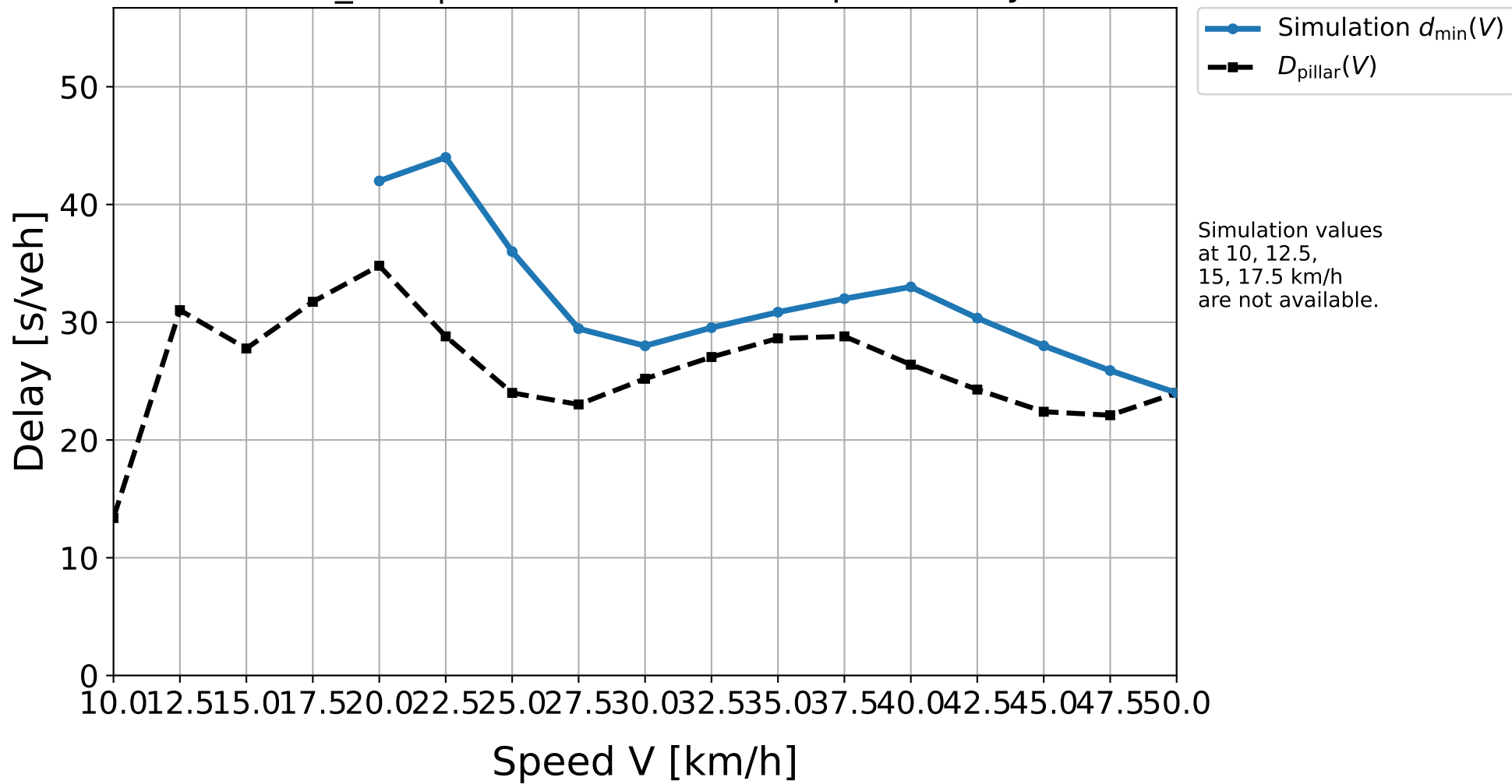
D10_H01 | Simulation result vs. pillar delay
