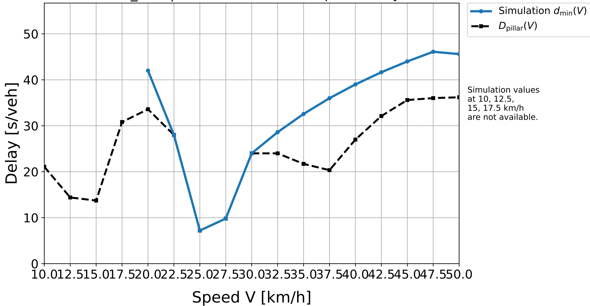
D30_H02 | Simulation result vs. pillar delay
