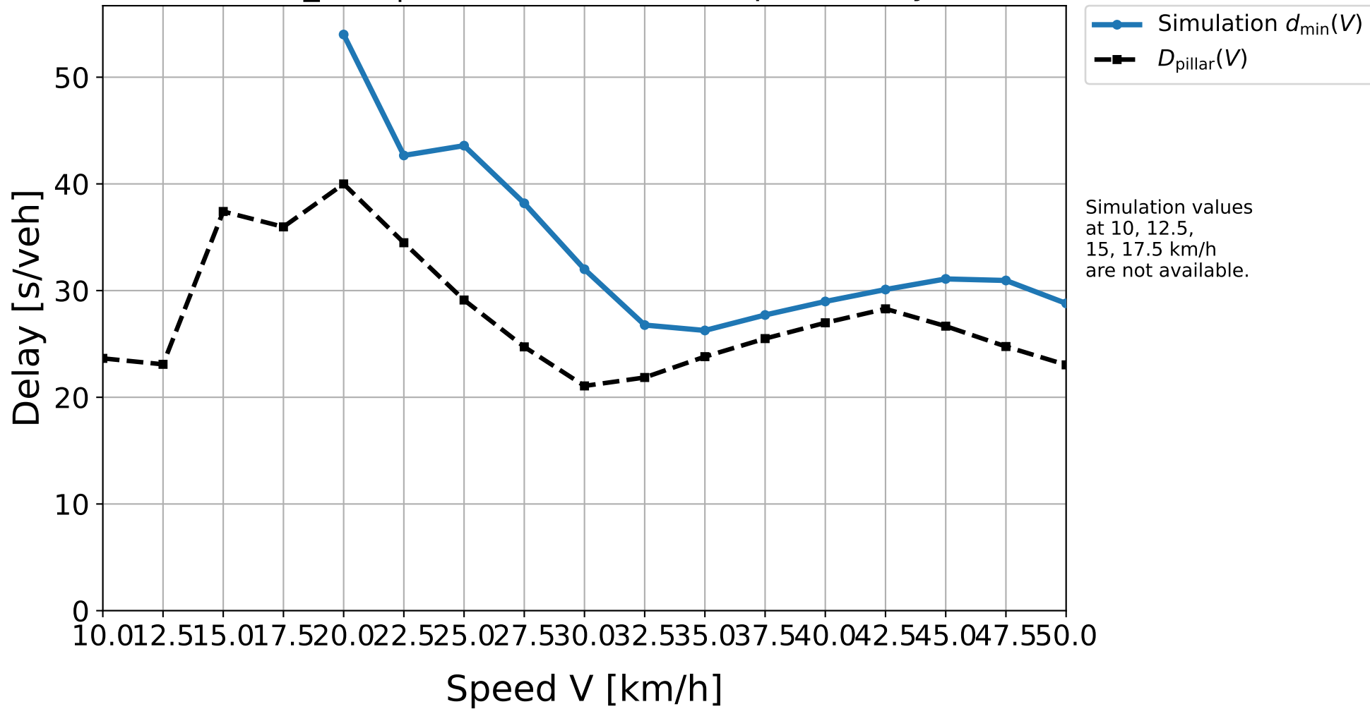
D10_H03 | Simulation result vs. pillar delay
