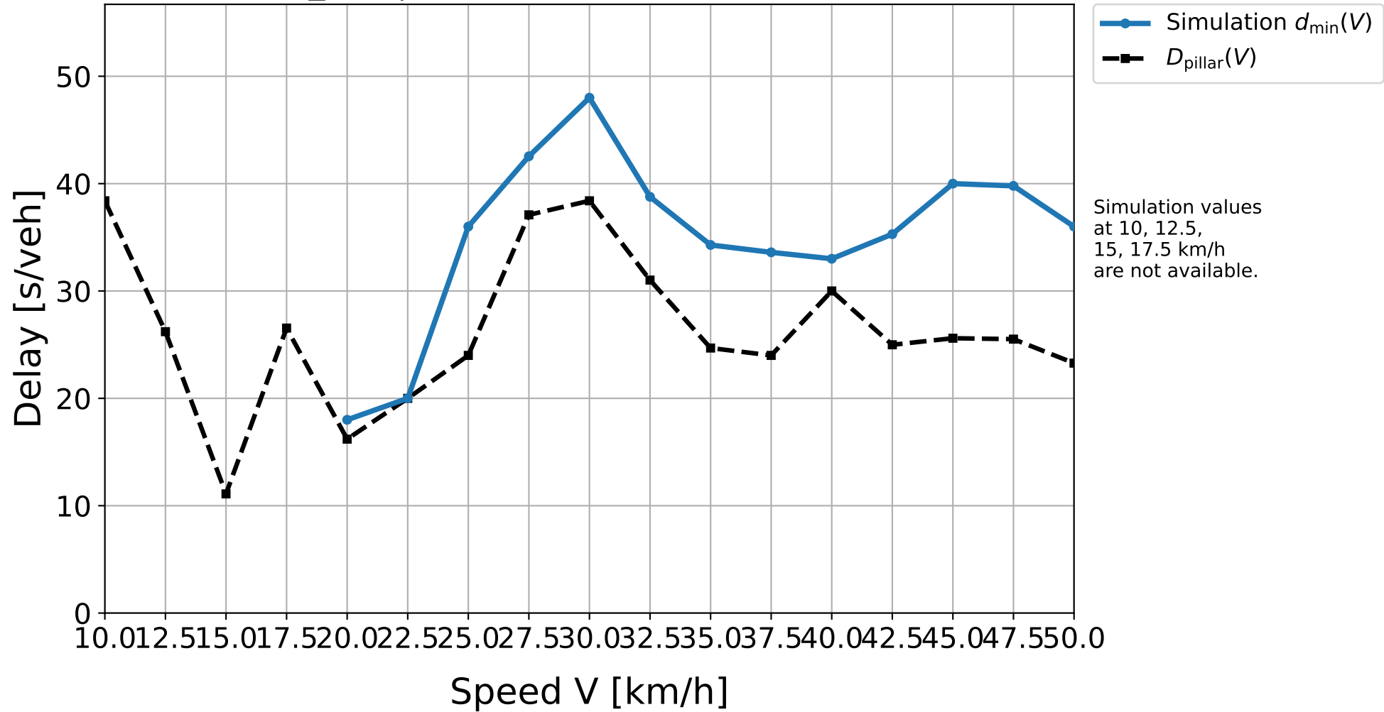
D30_314 | Simulation result vs. pillar delay
