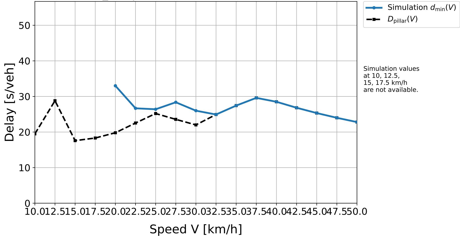
D10_334 | Simulation result vs. pillar delay
