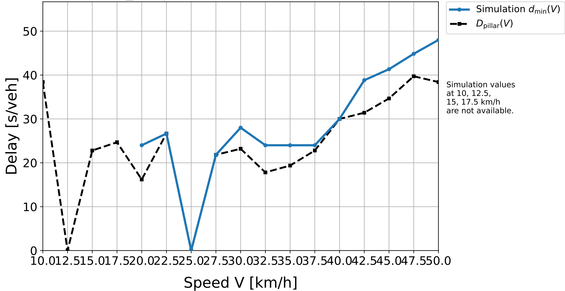
D50_321 | Simulation result vs. pillar delay
