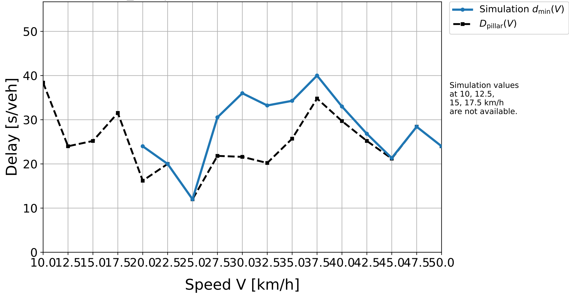
D50_324 | Simulation result vs. pillar delay
