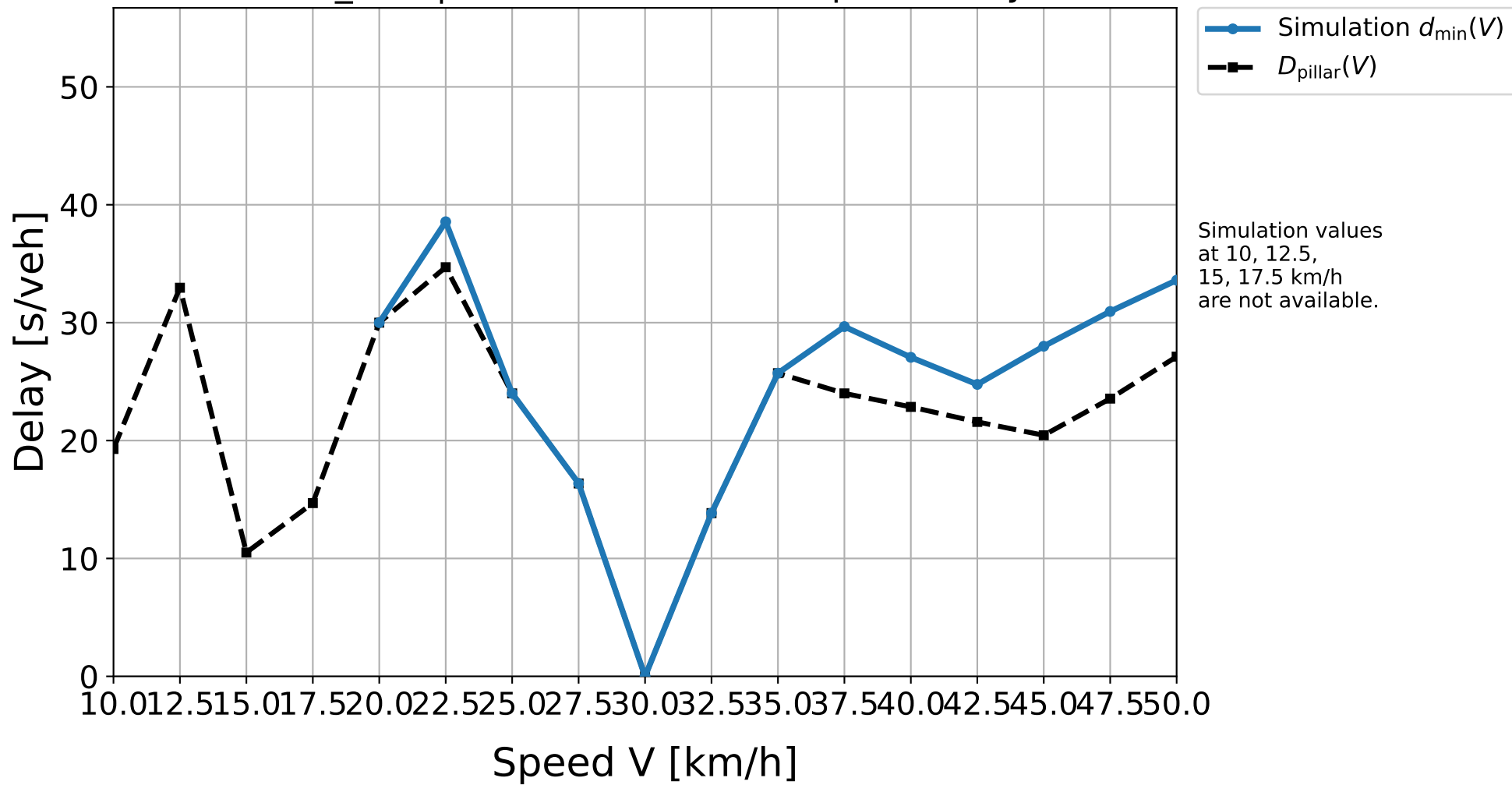
D30_H07 | Simulation result vs. pillar delay
