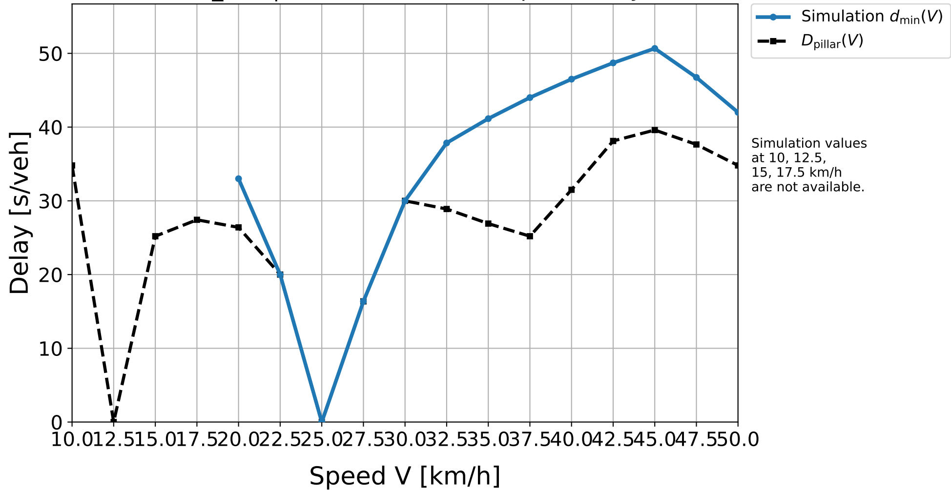
D50_331 | Simulation result vs. pillar delay
