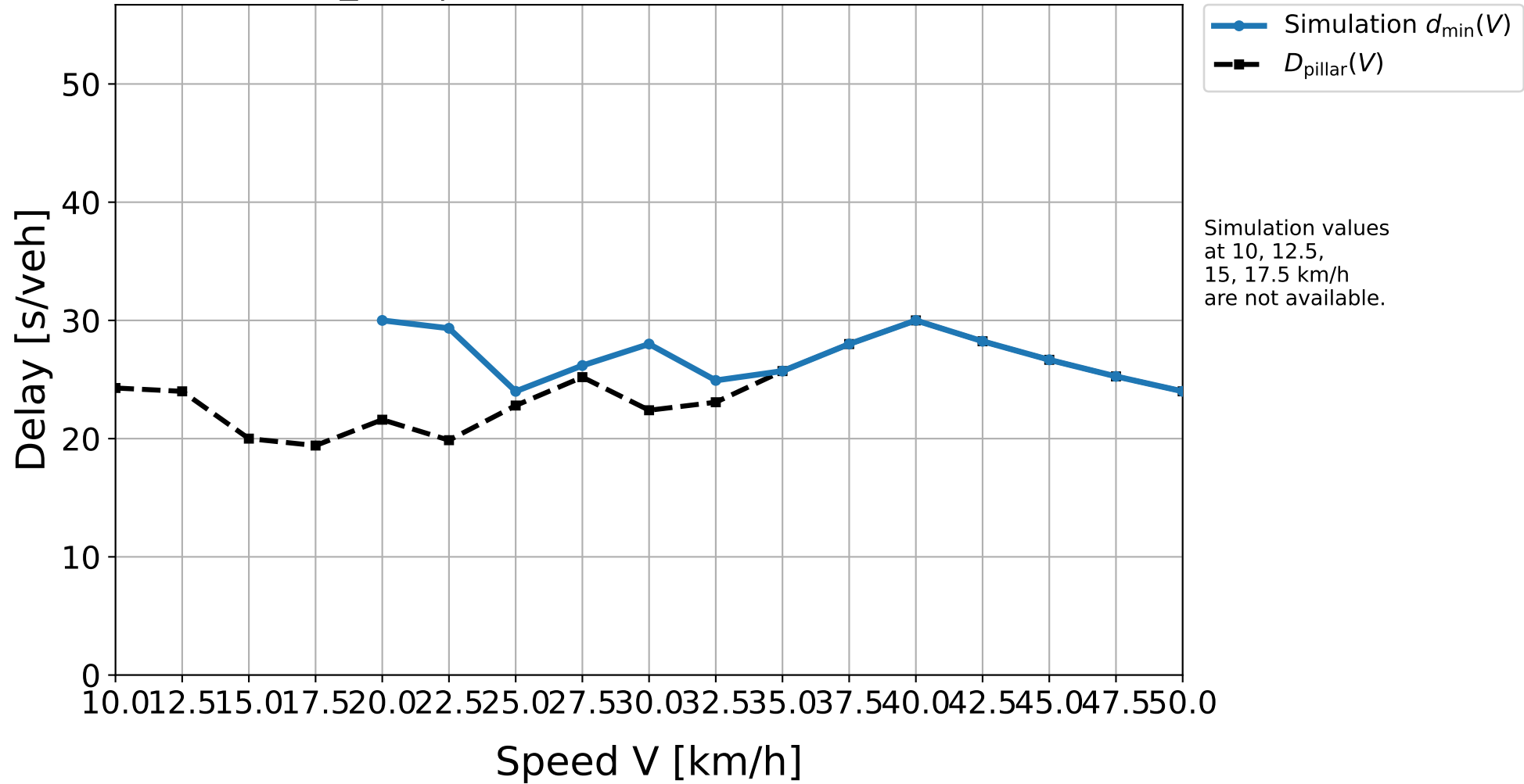
D10_314 | Simulation result vs. pillar delay
