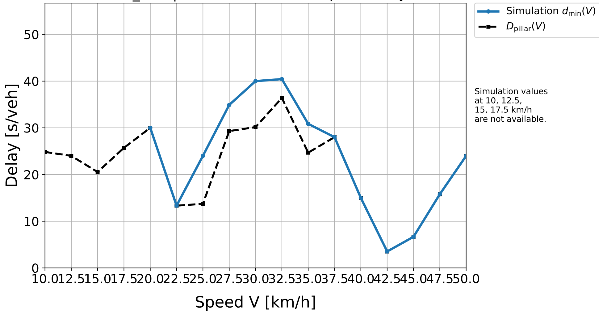
D50_H02 | Simulation result vs. pillar delay
