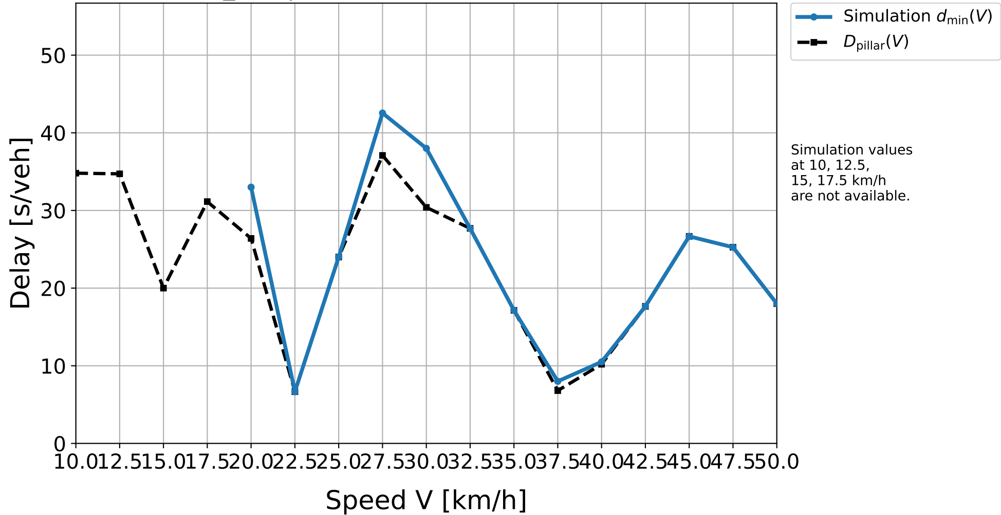
D50_333 | Simulation result vs. pillar delay
