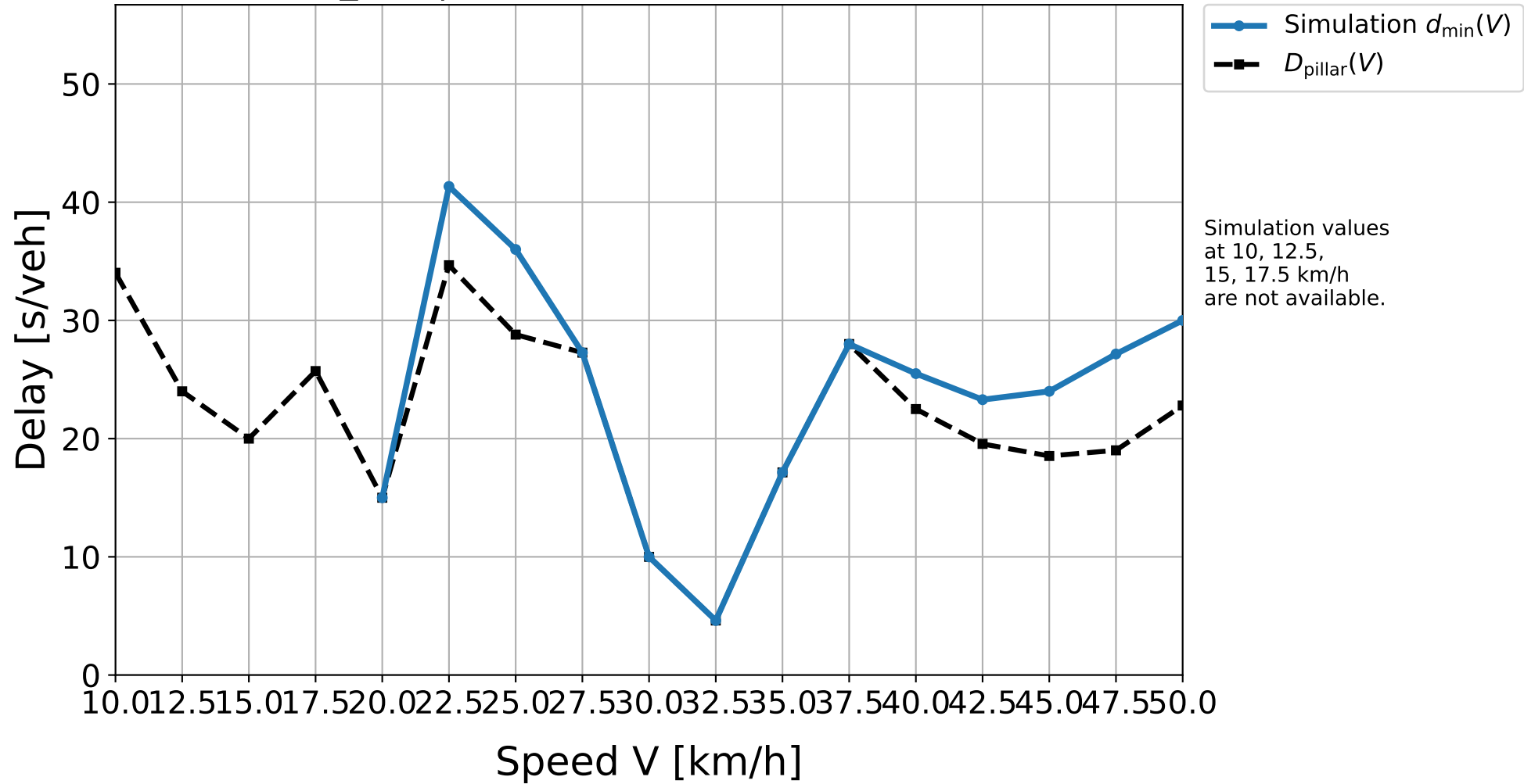
D50_332 | Simulation result vs. pillar delay
