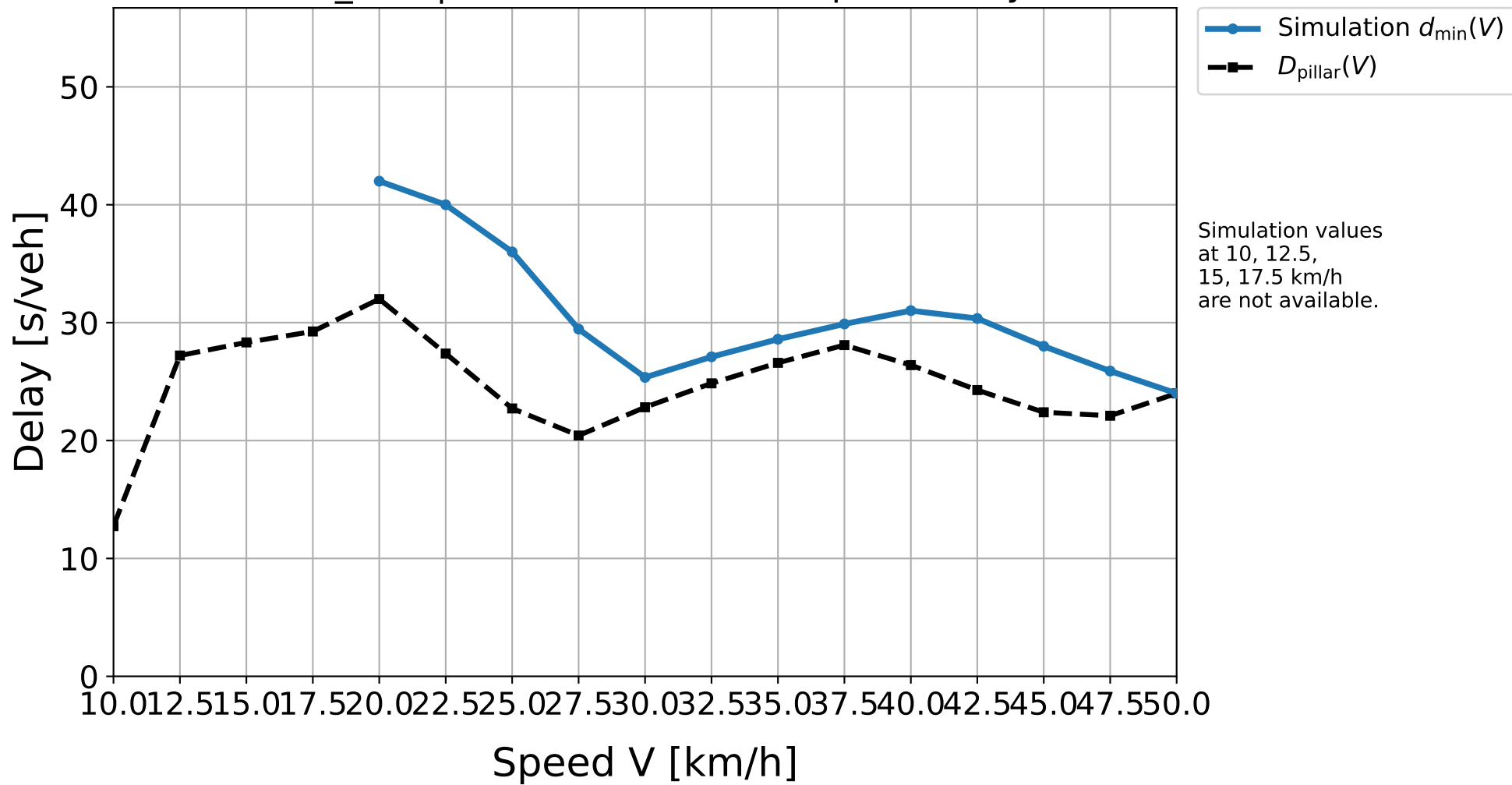
D10_H06 | Simulation result vs. pillar delay
