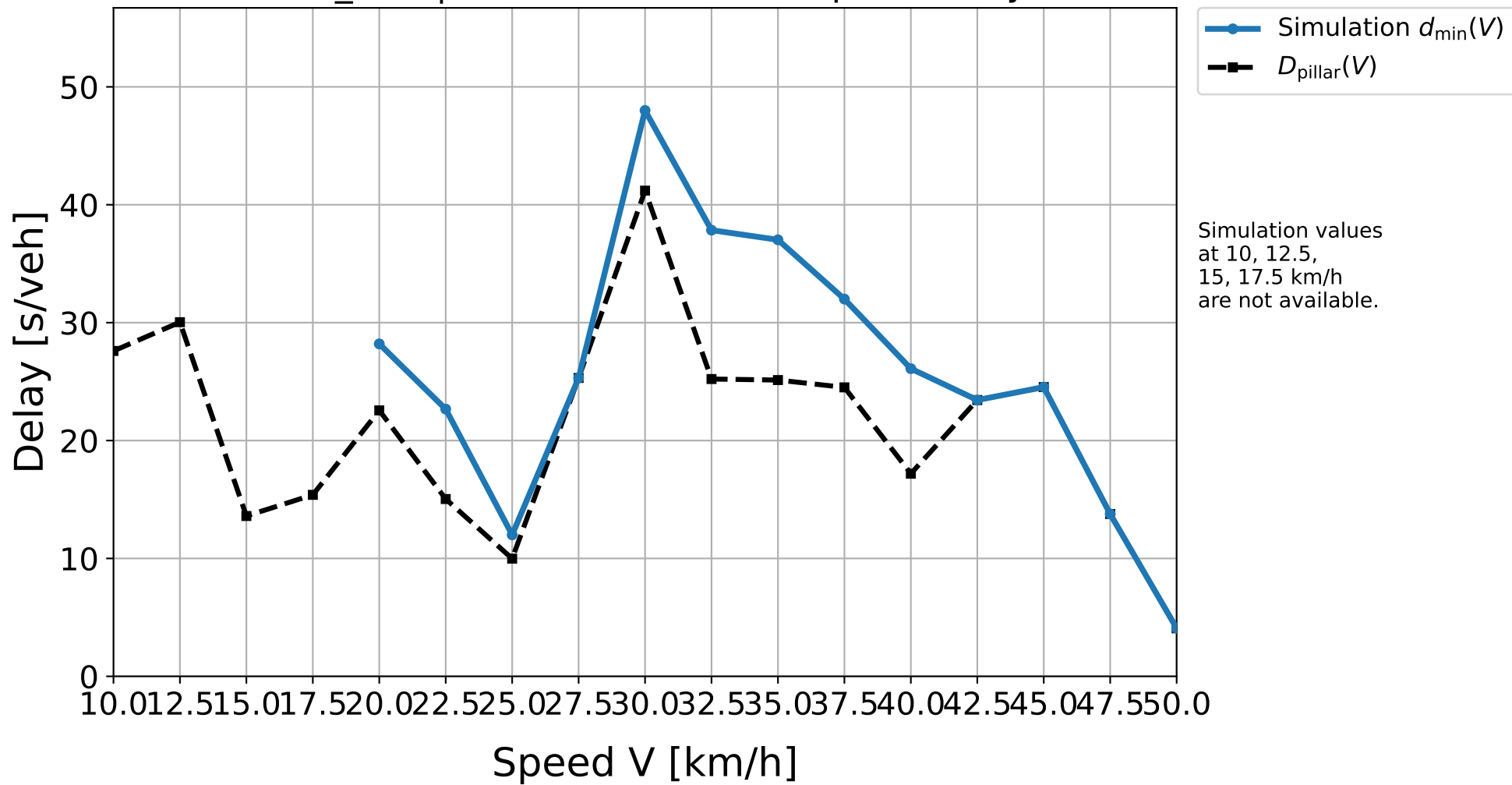
D50_H04 | Simulation result vs. pillar delay
