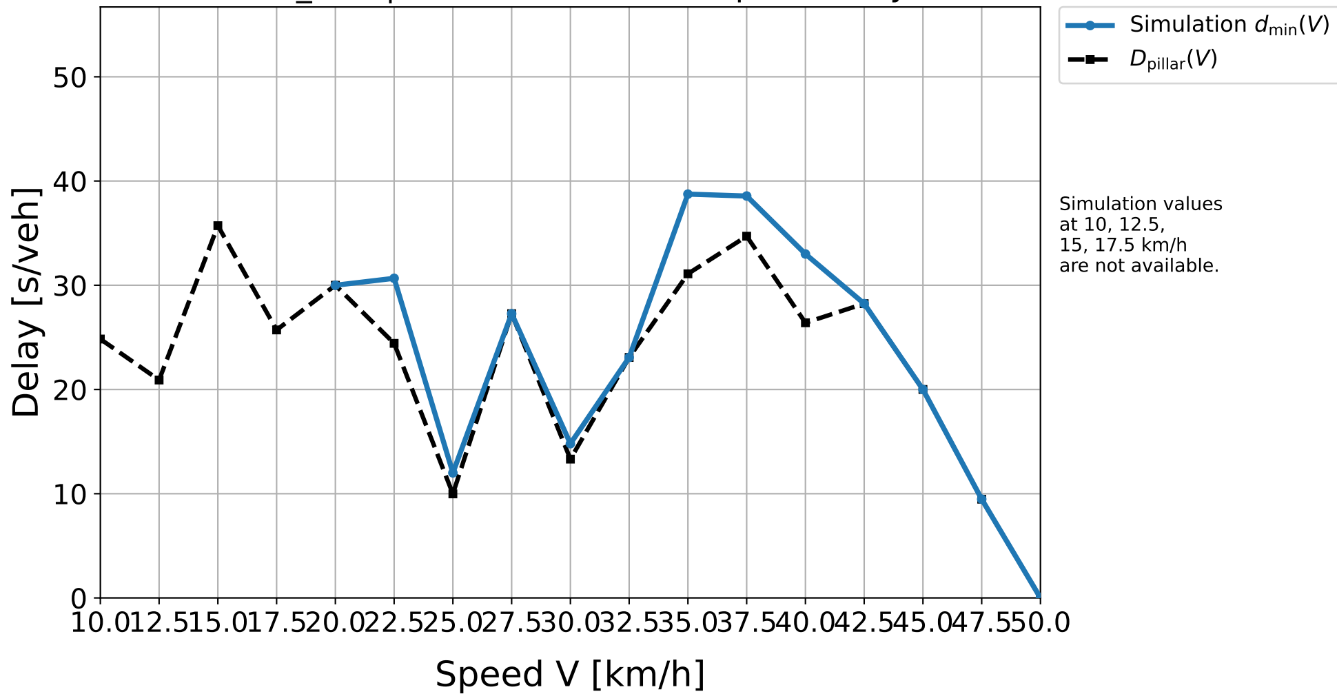
D50_H07 | Simulation result vs. pillar delay
