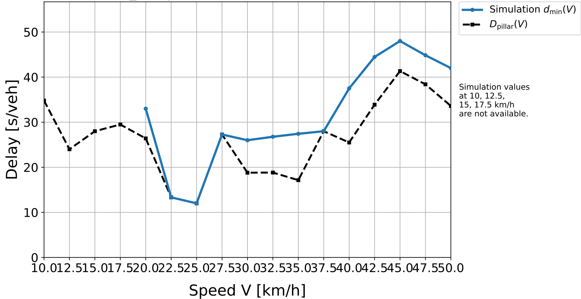
D50_334 | Simulation result vs. pillar delay
