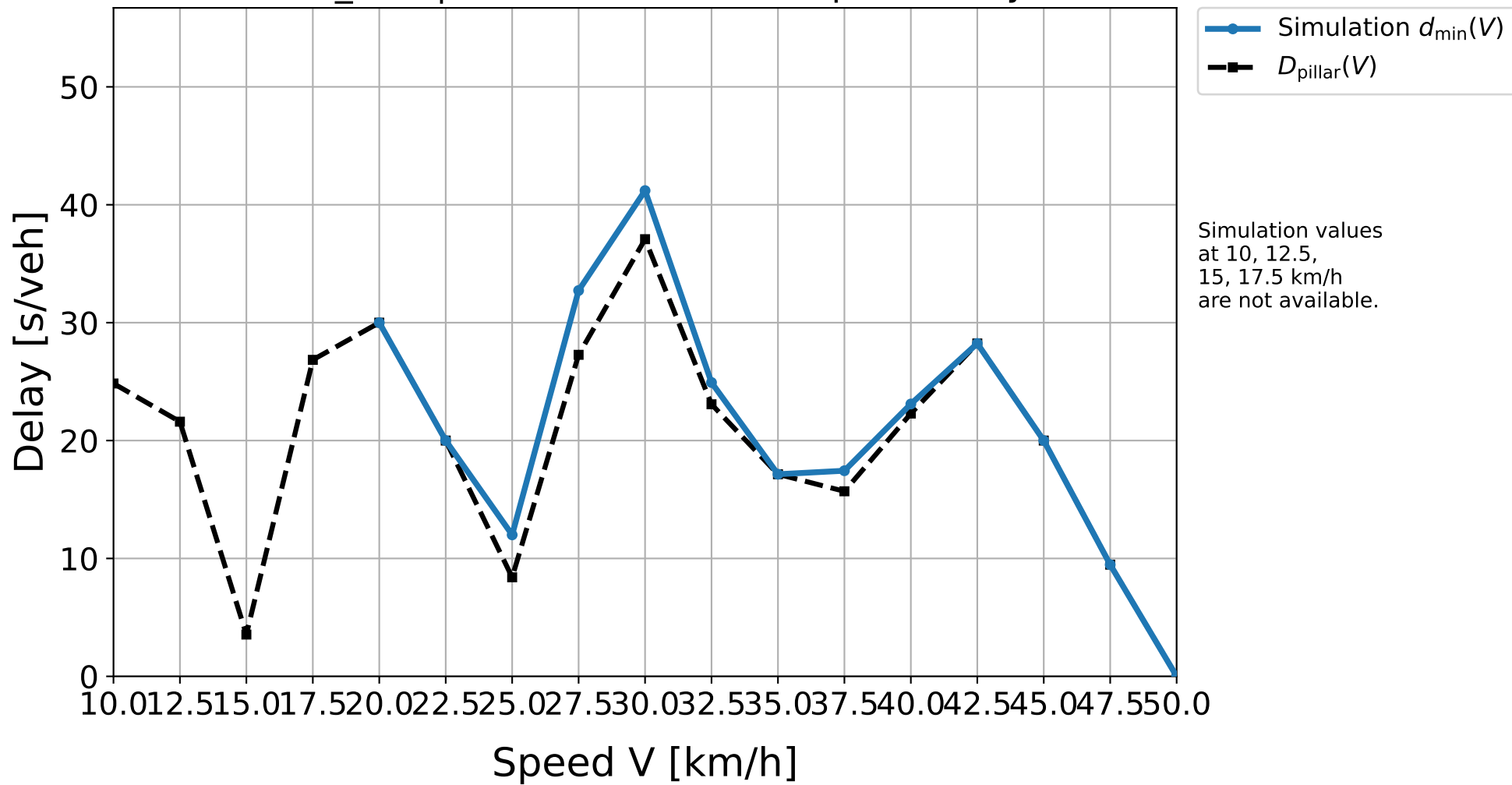
D50_H06 | Simulation result vs. pillar delay
