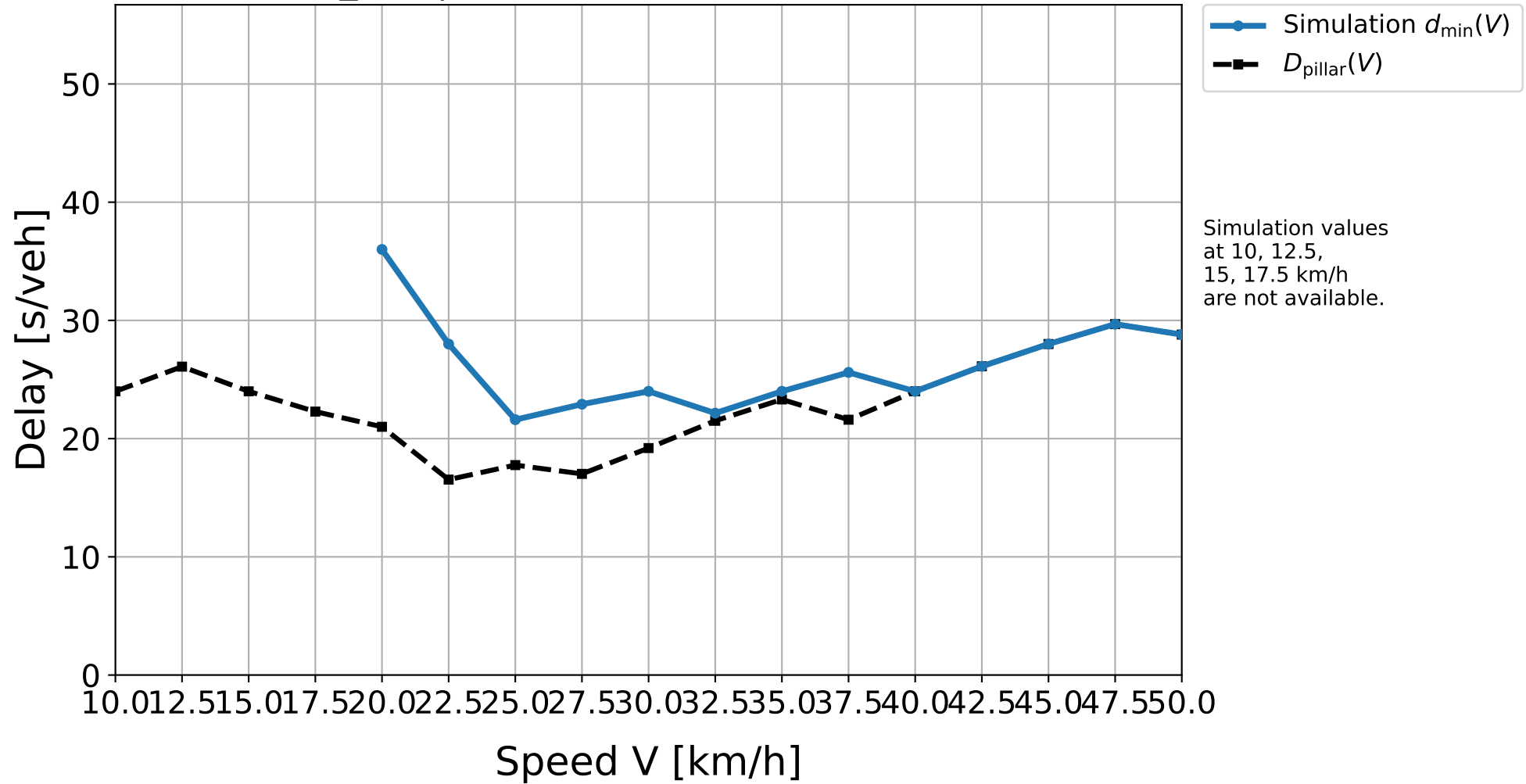
D10_324 | Simulation result vs. pillar delay
