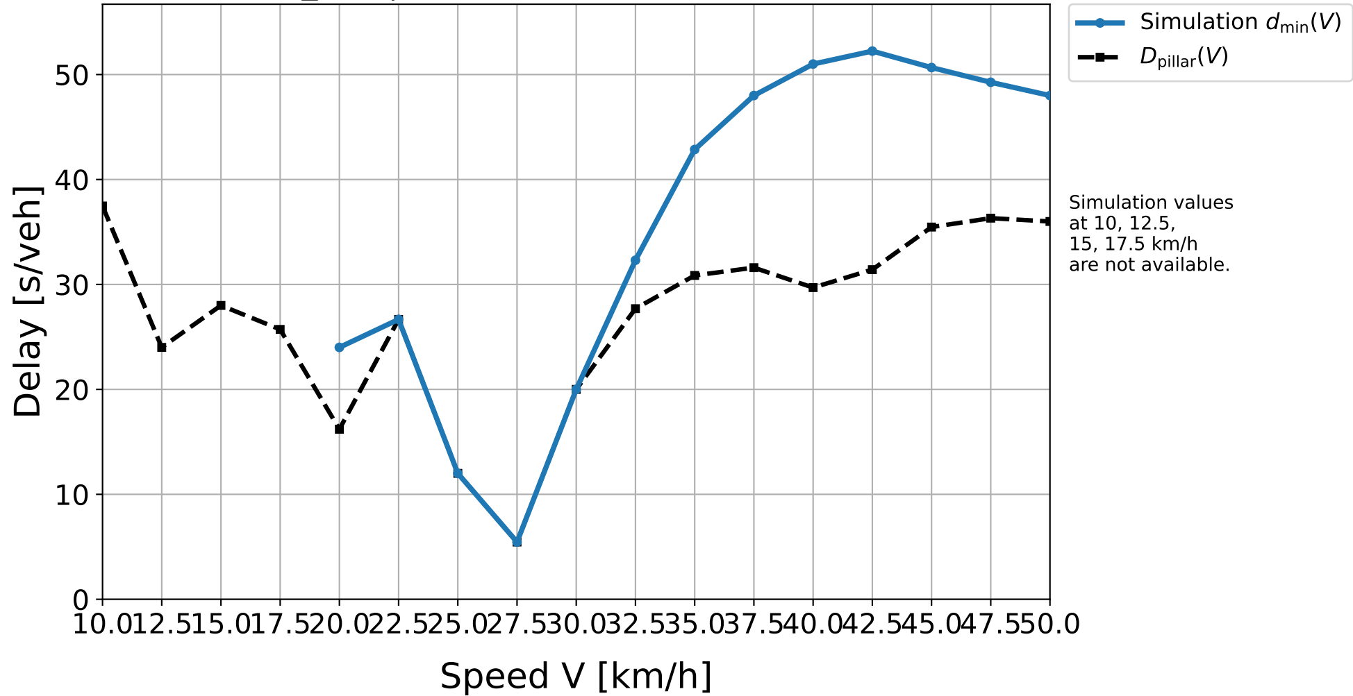
D50_311 | Simulation result vs. pillar delay
