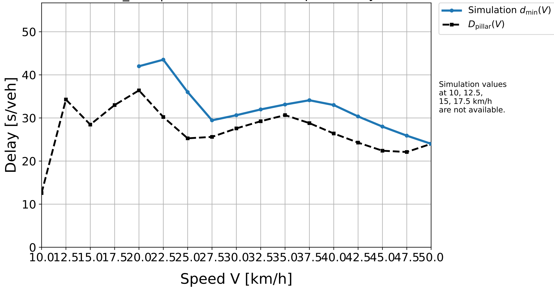
D10_H07 | Simulation result vs. pillar delay
