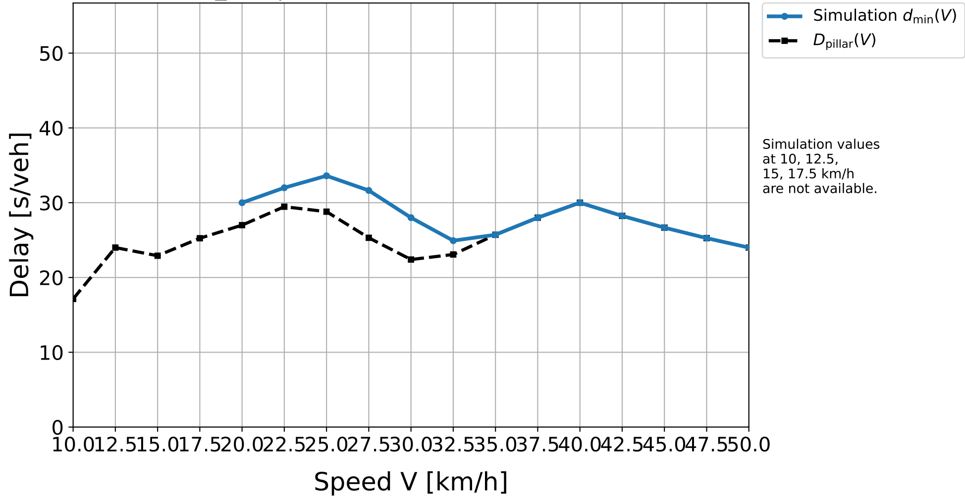
D10_312 | Simulation result vs. pillar delay
