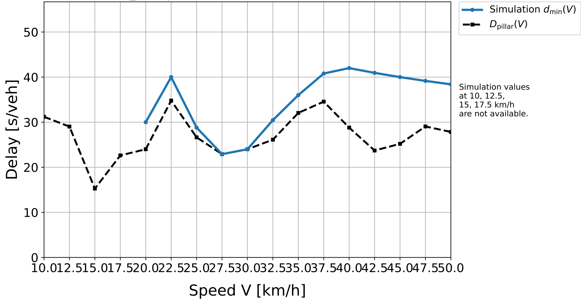
D30_324 | Simulation result vs. pillar delay
