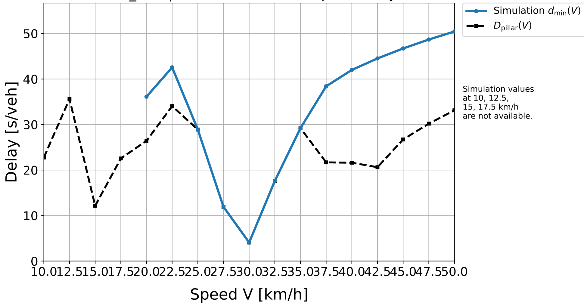
D30_H05 | Simulation result vs. pillar delay
