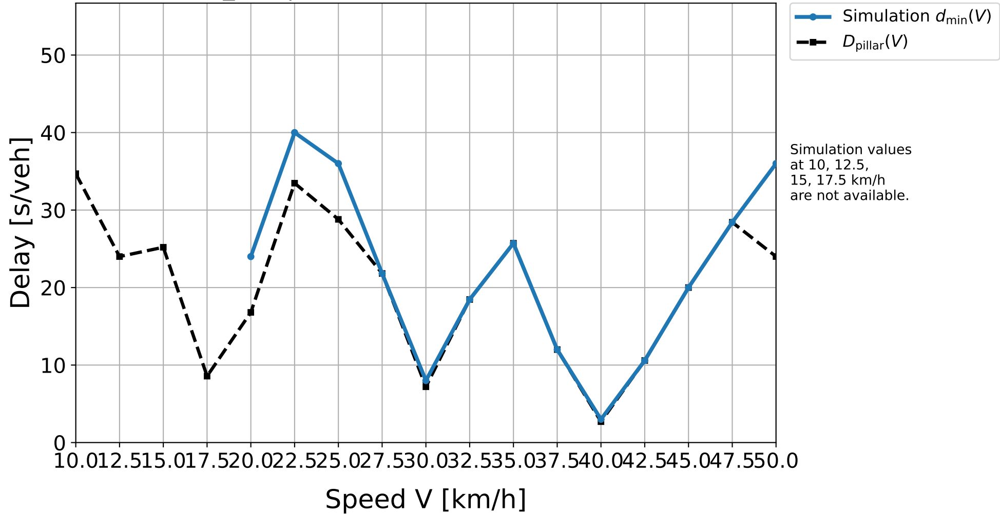
D50_322 | Simulation result vs. pillar delay
