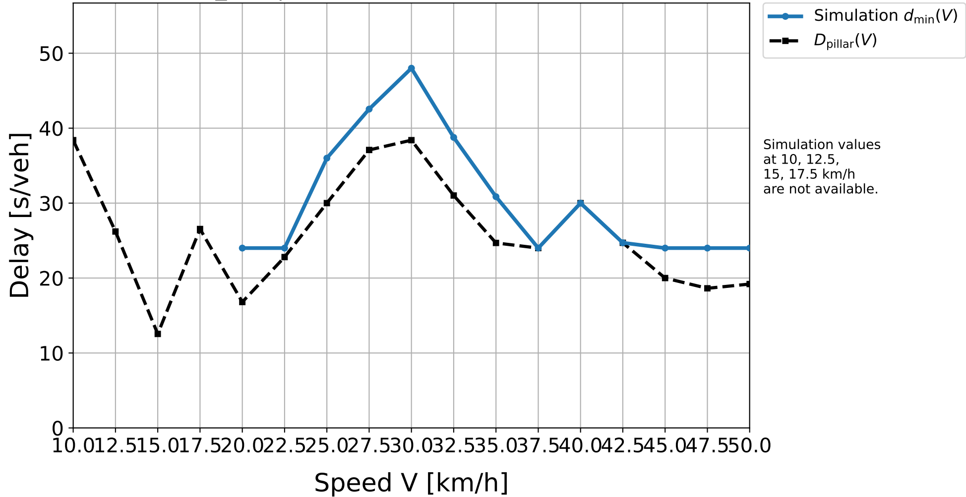
D30_321 | Simulation result vs. pillar delay
