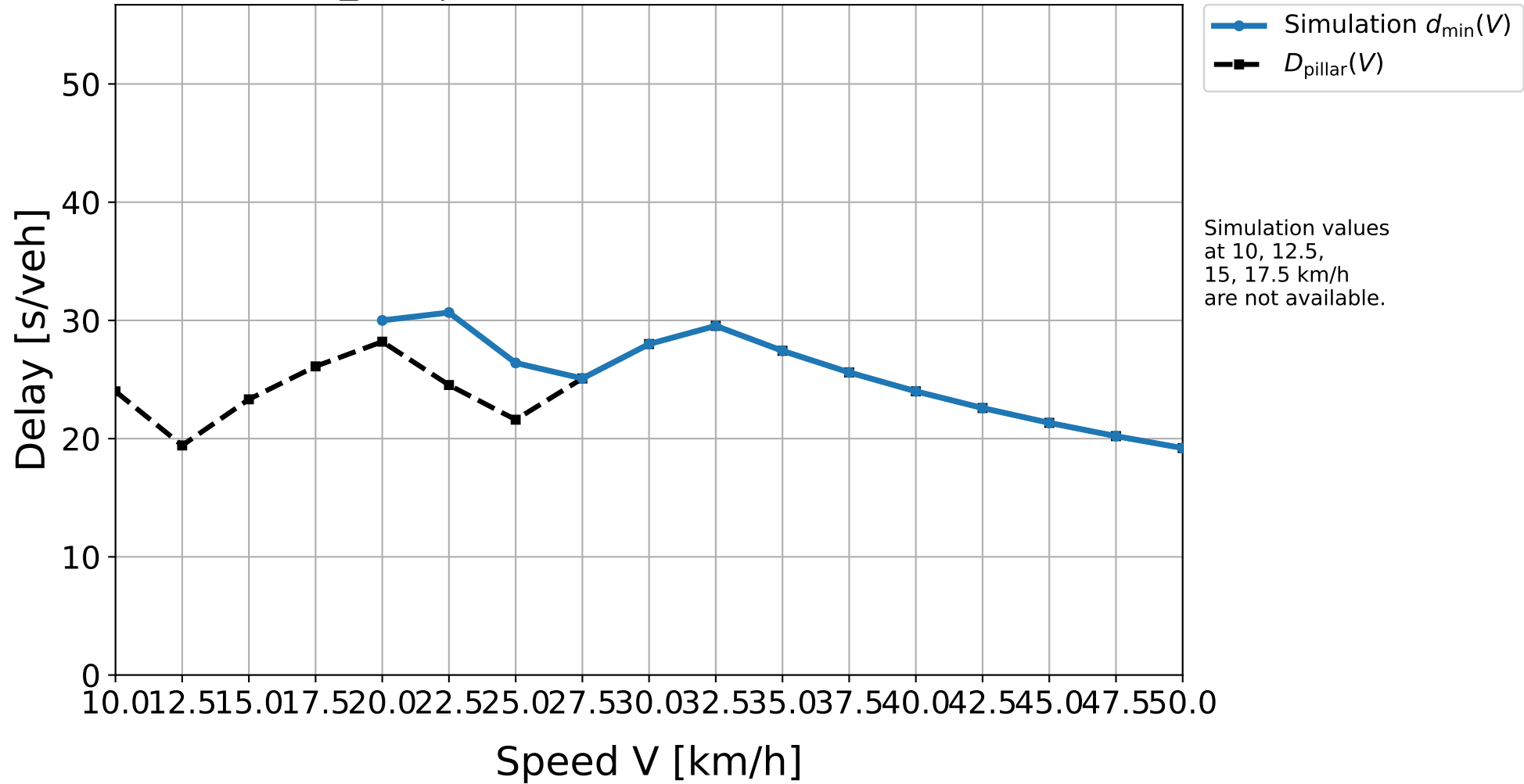
D10_311 | Simulation result vs. pillar delay
