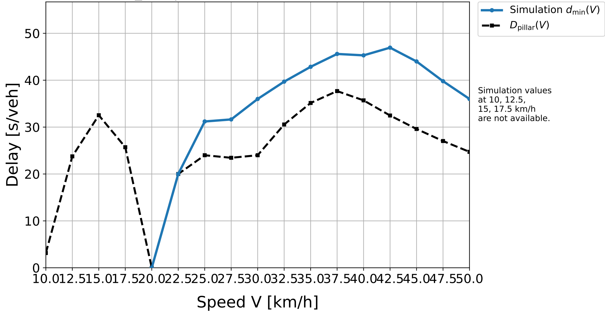
D30_312 | Simulation result vs. pillar delay
