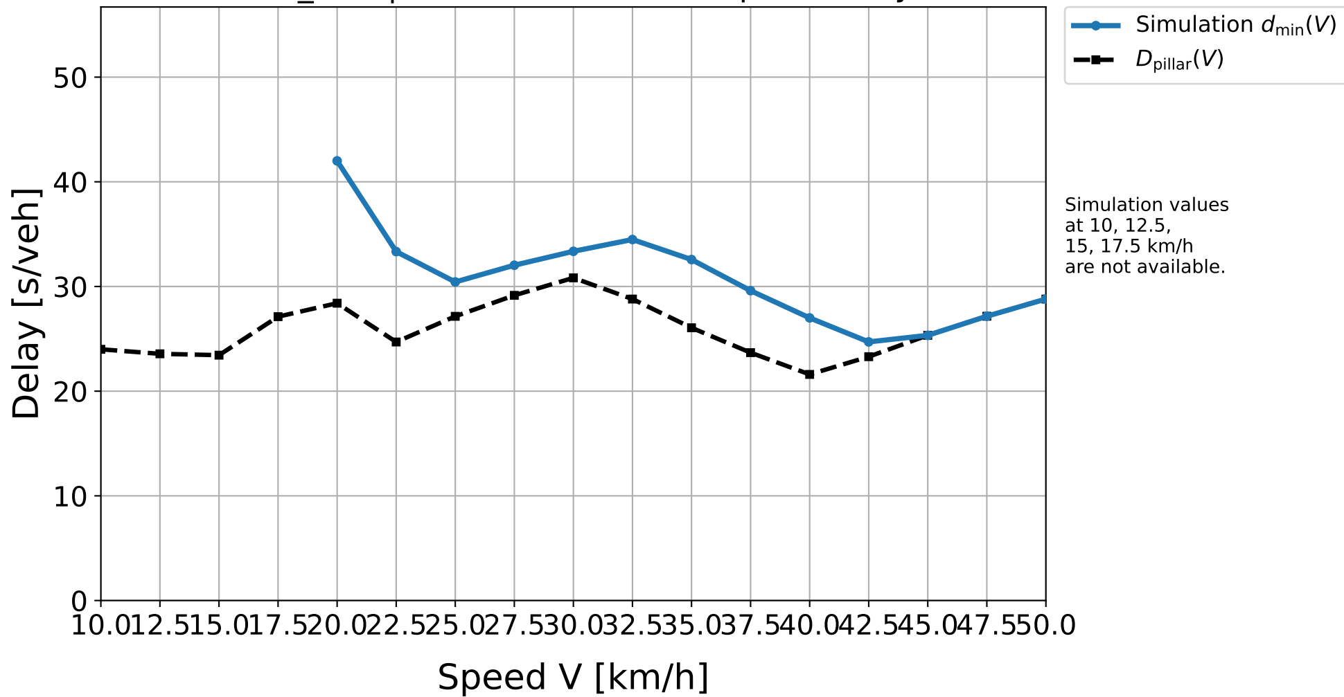
D10_H02 | Simulation result vs. pillar delay
