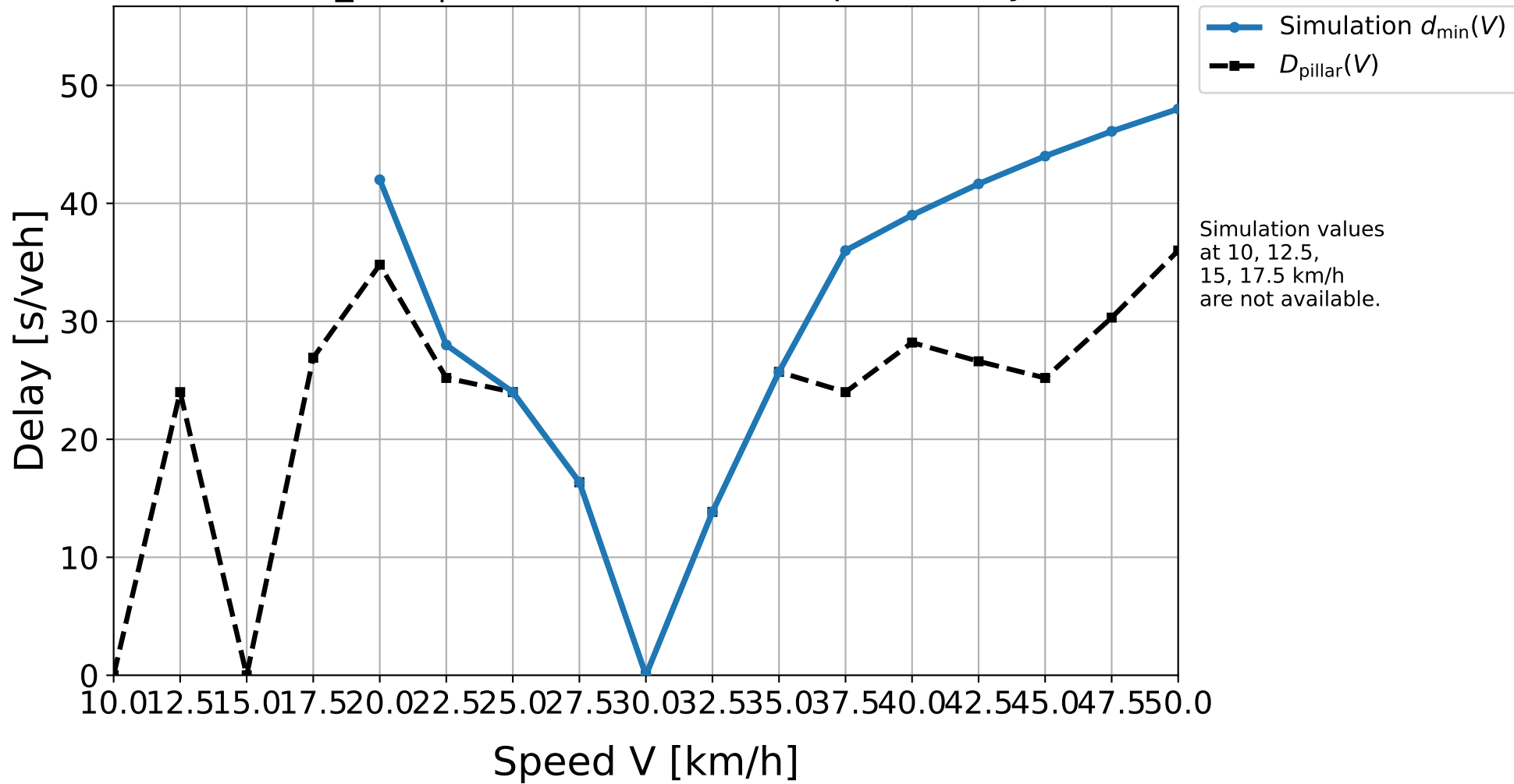
D30_H01 | Simulation result vs. pillar delay
