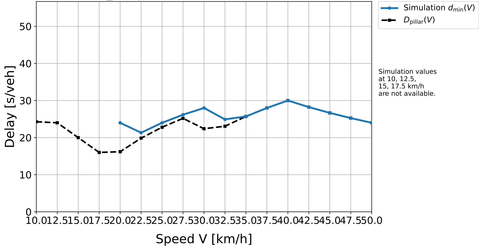
D10_321 | Simulation result vs. pillar delay
