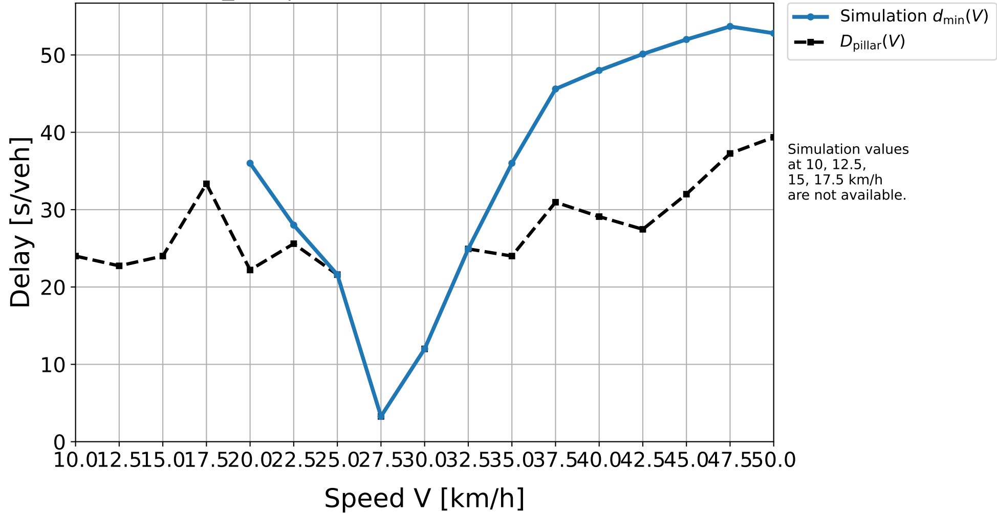
D30_323 | Simulation result vs. pillar delay
