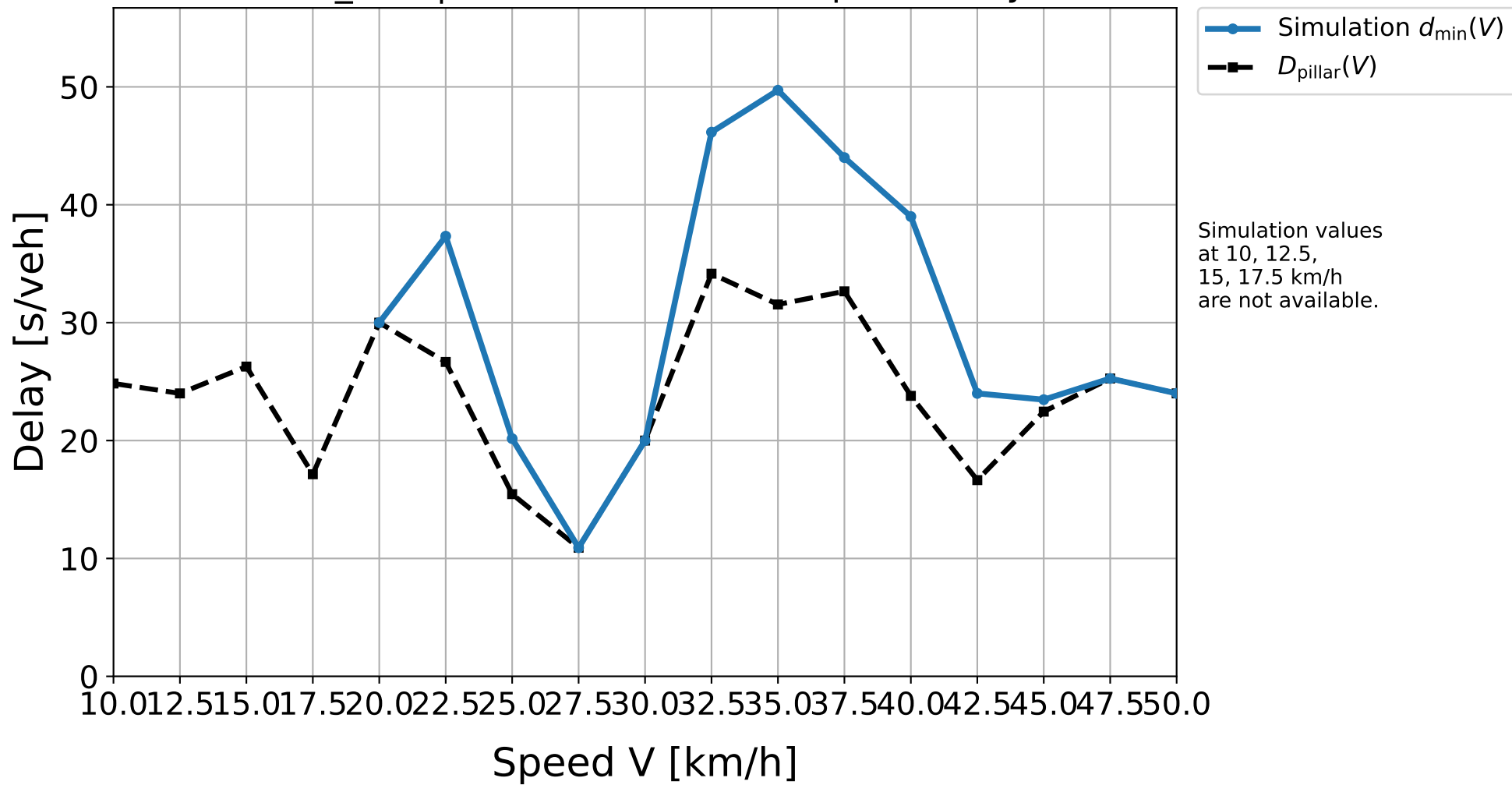
D50_H03 | Simulation result vs. pillar delay
