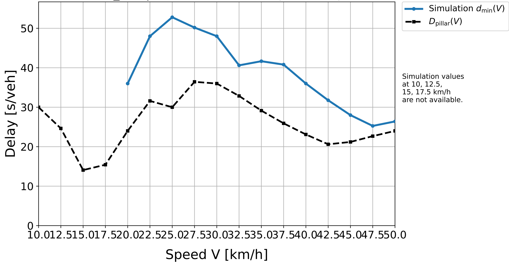
D30_311 | Simulation result vs. pillar delay
