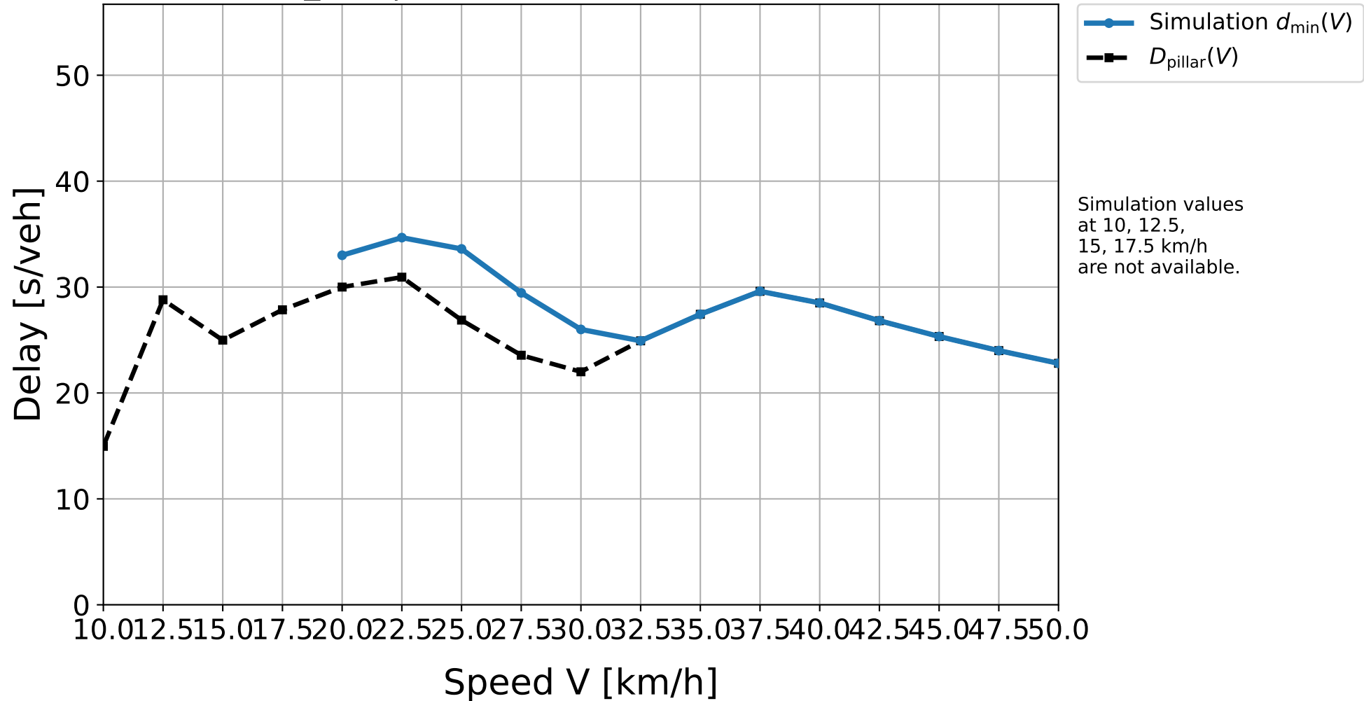
D10_332 | Simulation result vs. pillar delay
