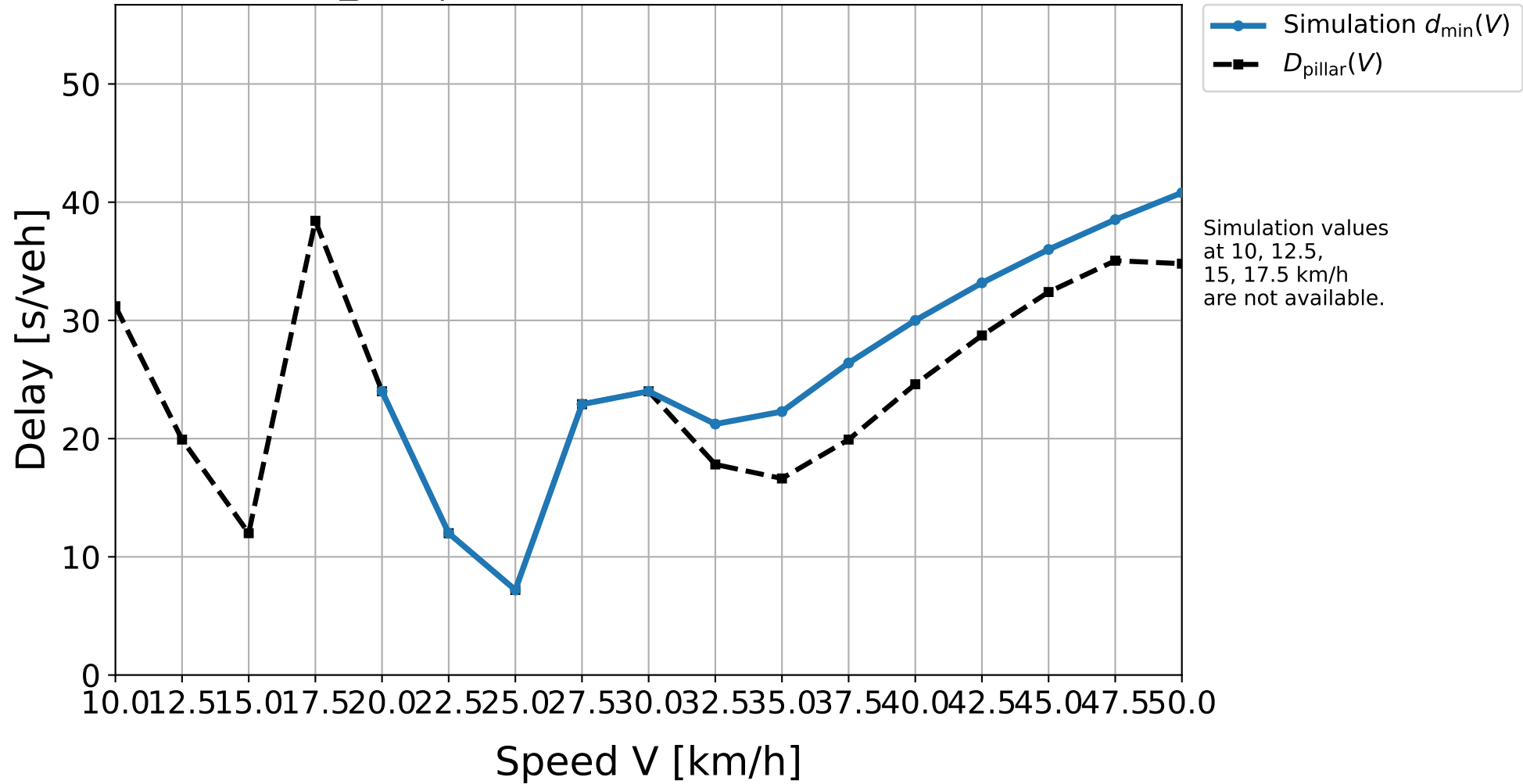
D30_313 | Simulation result vs. pillar delay
