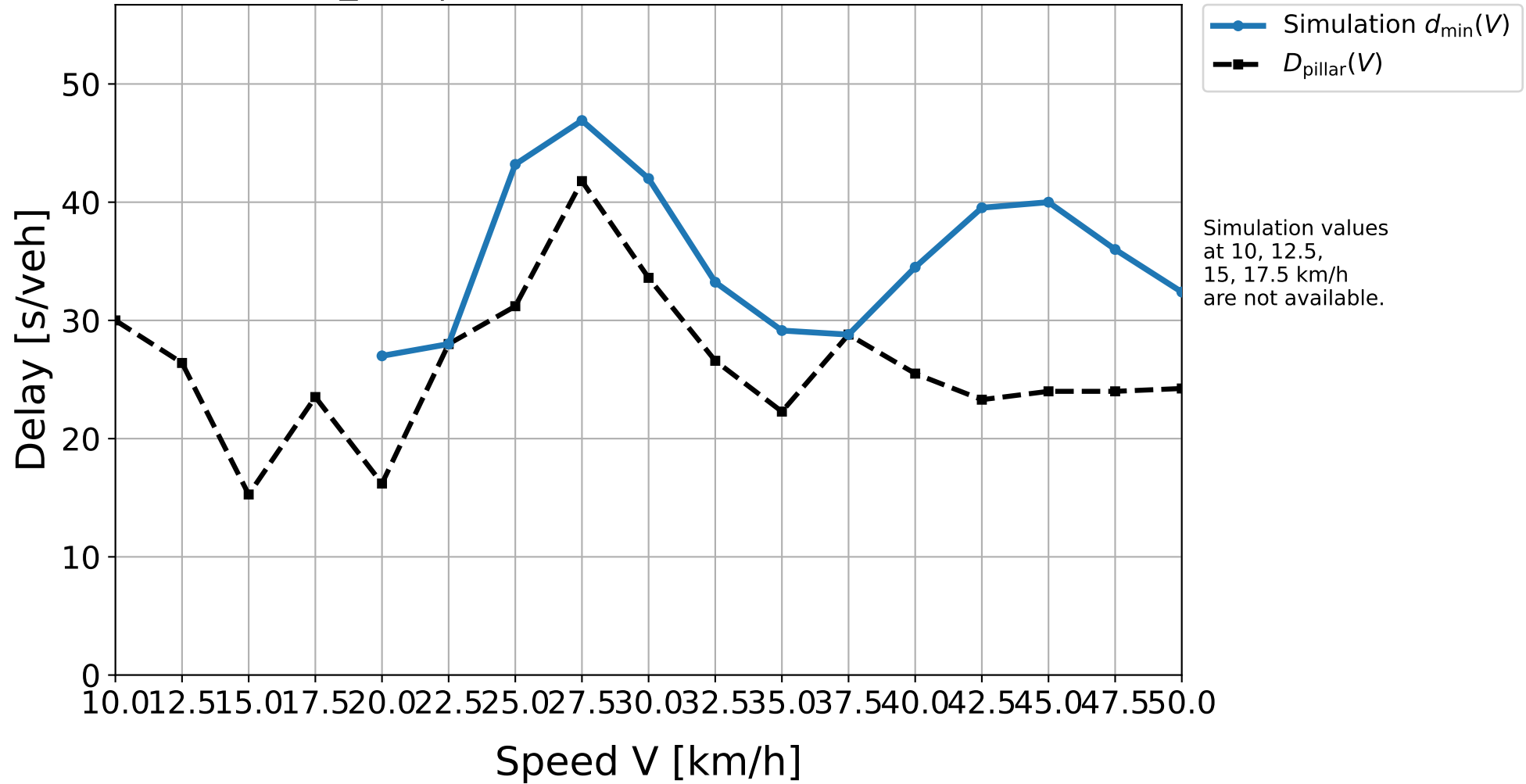
D30_334 | Simulation result vs. pillar delay
