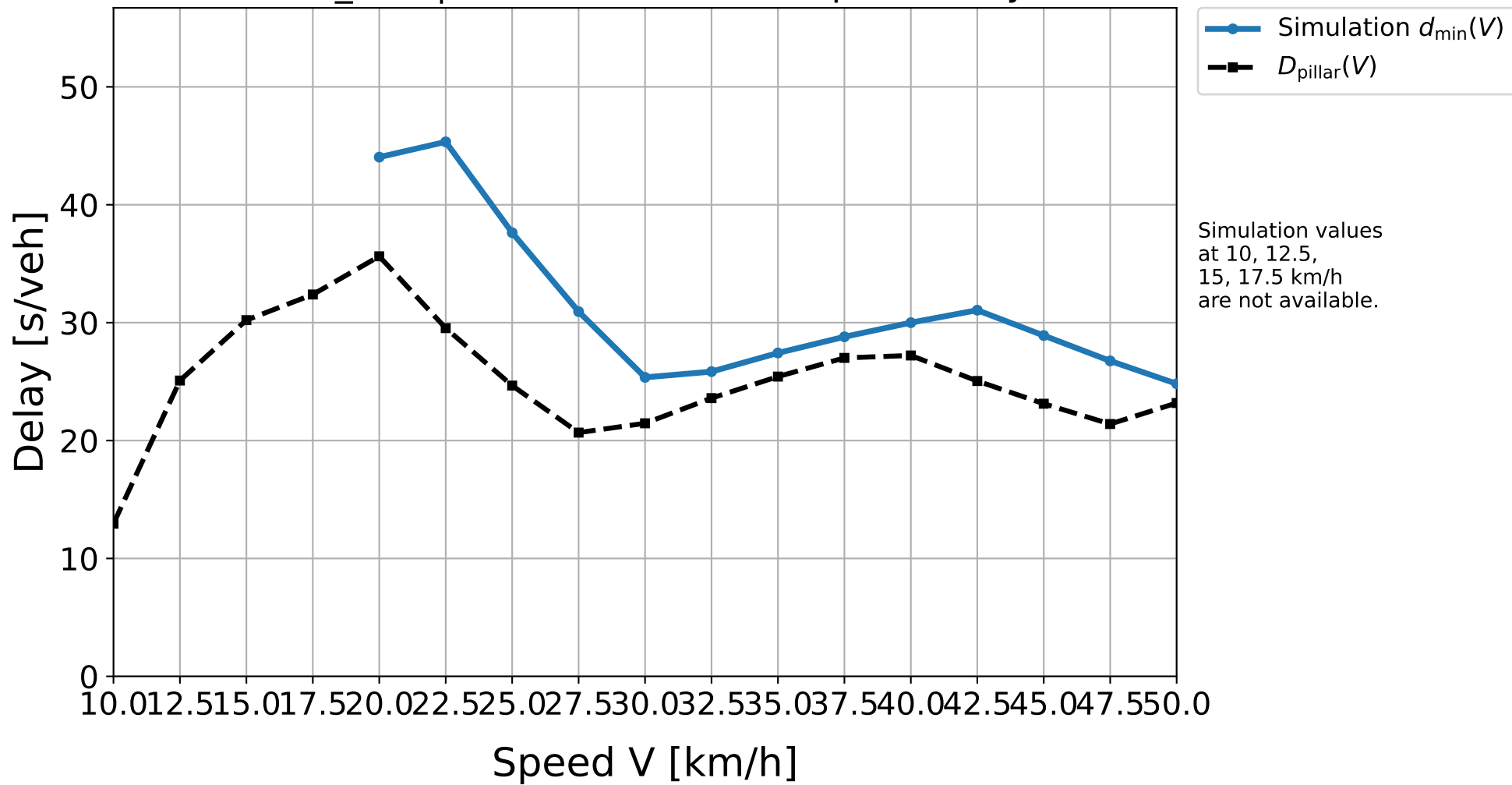
D10_H04 | Simulation result vs. pillar delay
