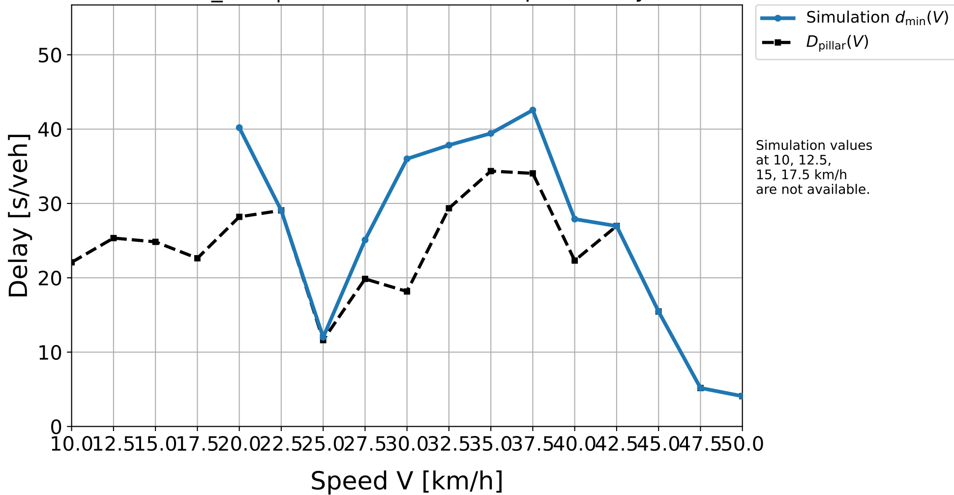
D50_H05 | Simulation result vs. pillar delay
