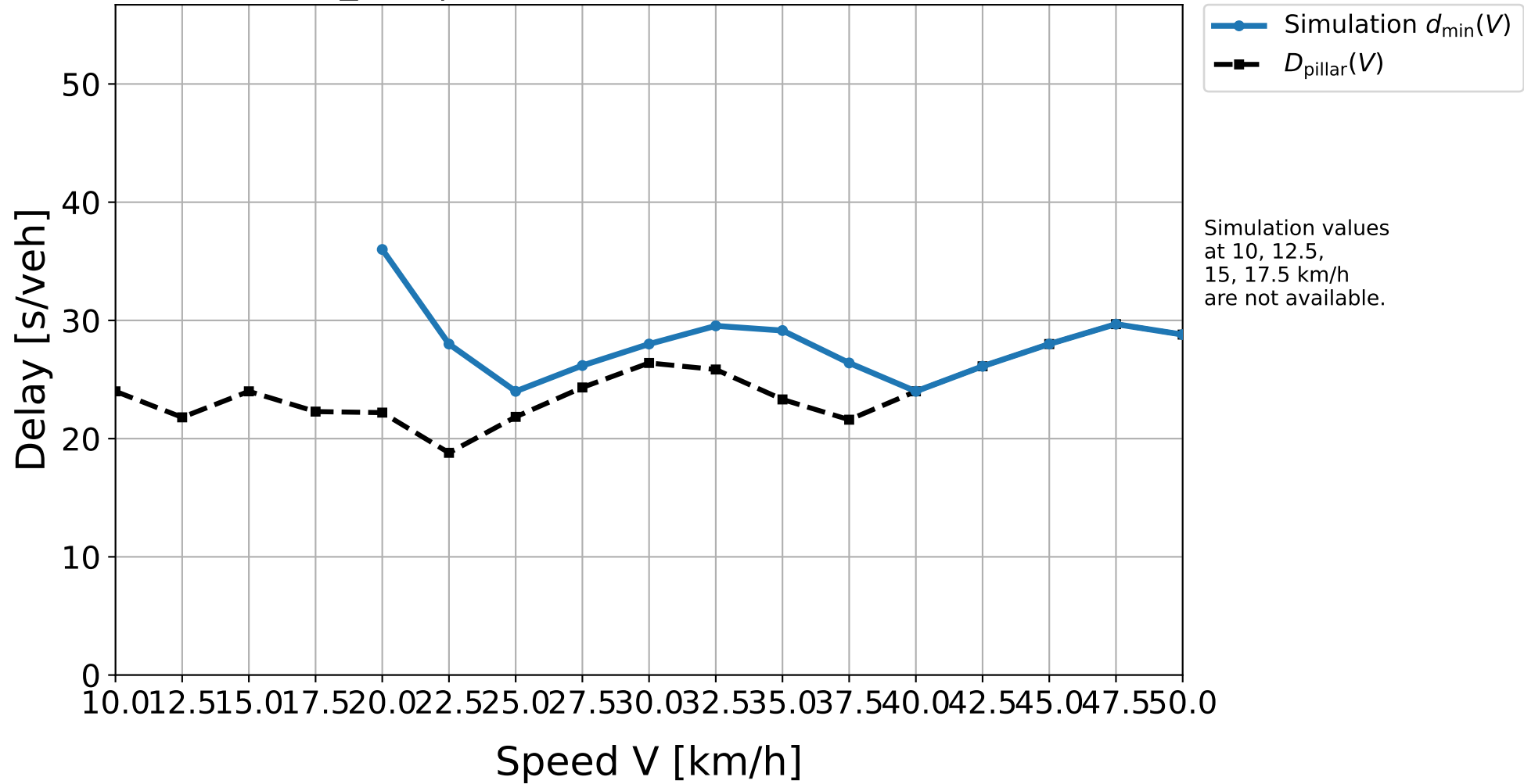
D10_322 | Simulation result vs. pillar delay
