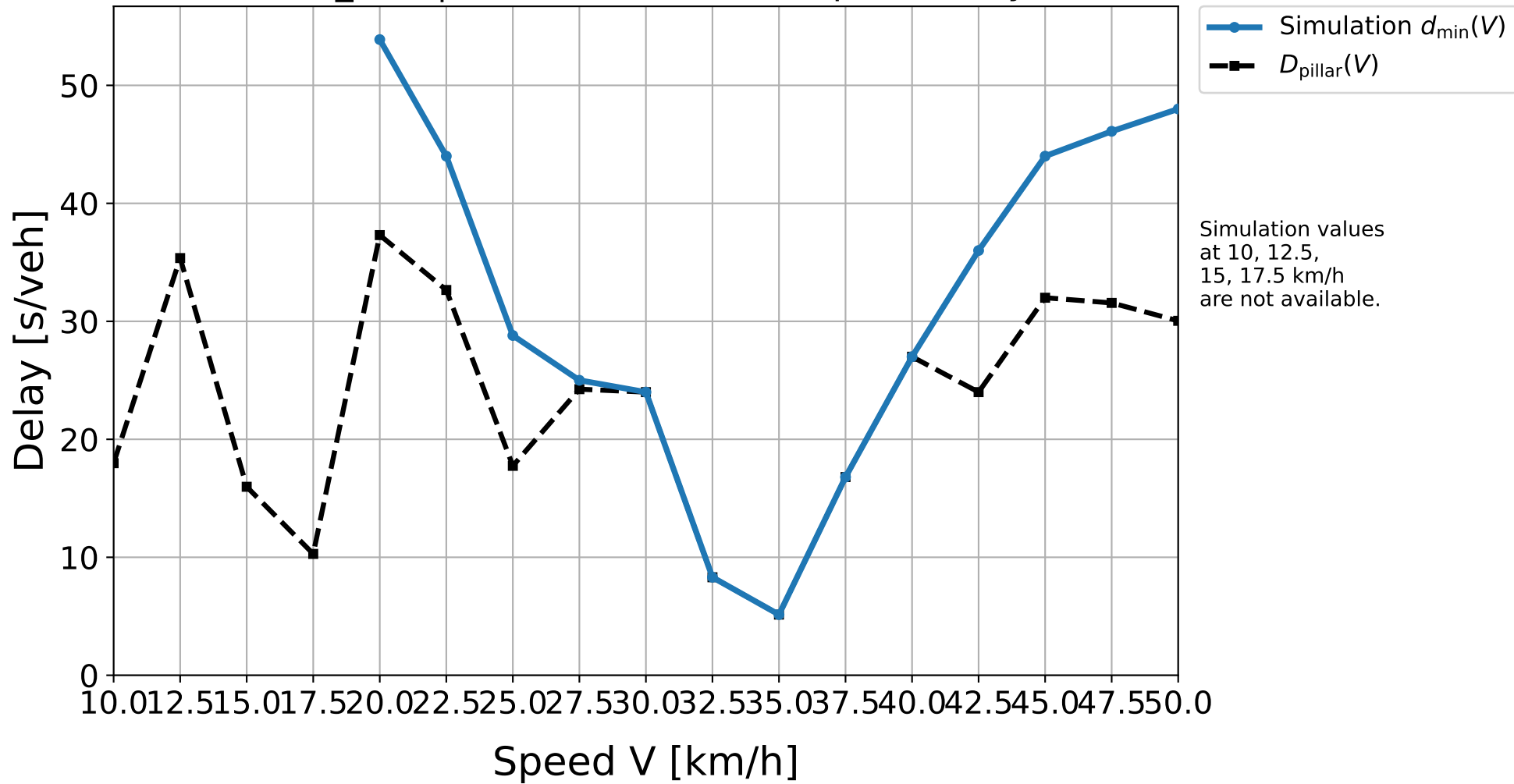
D30_H03 | Simulation result vs. pillar delay
