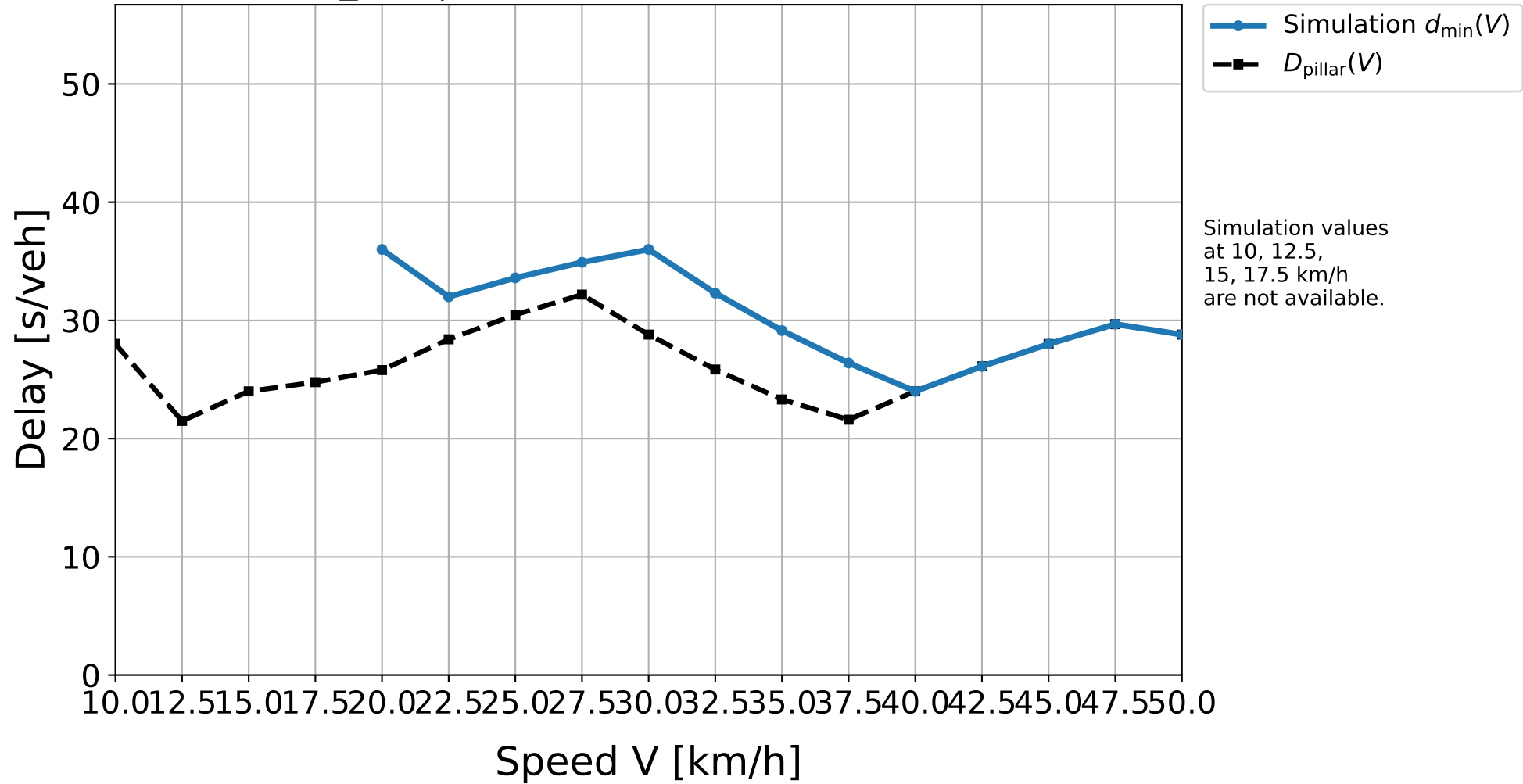
D10_313 | Simulation result vs. pillar delay
