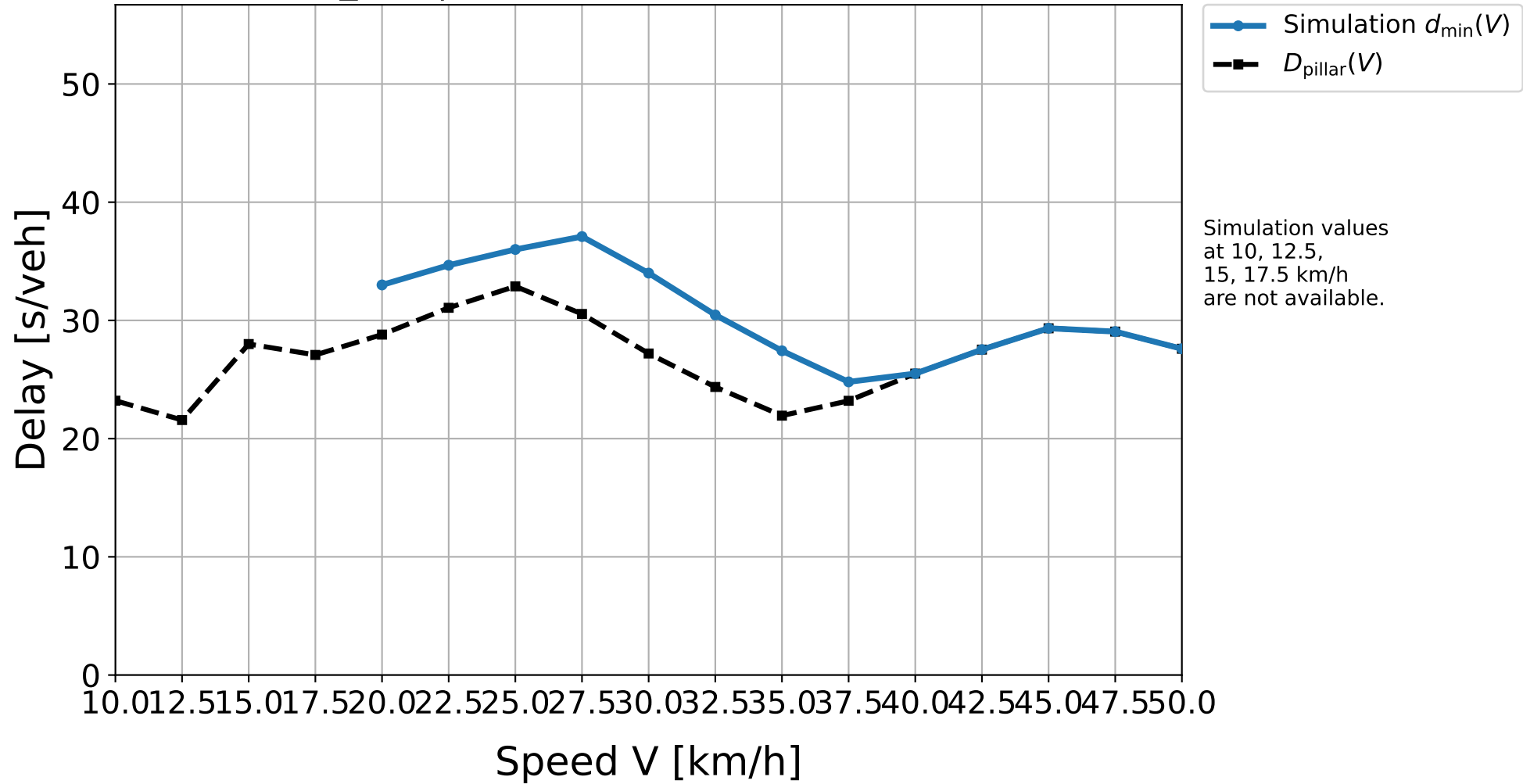
D10_333 | Simulation result vs. pillar delay
