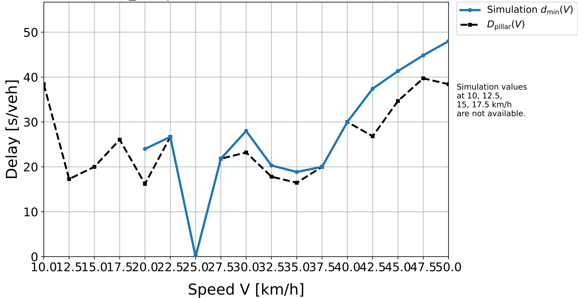
D50_314 | Simulation result vs. pillar delay
