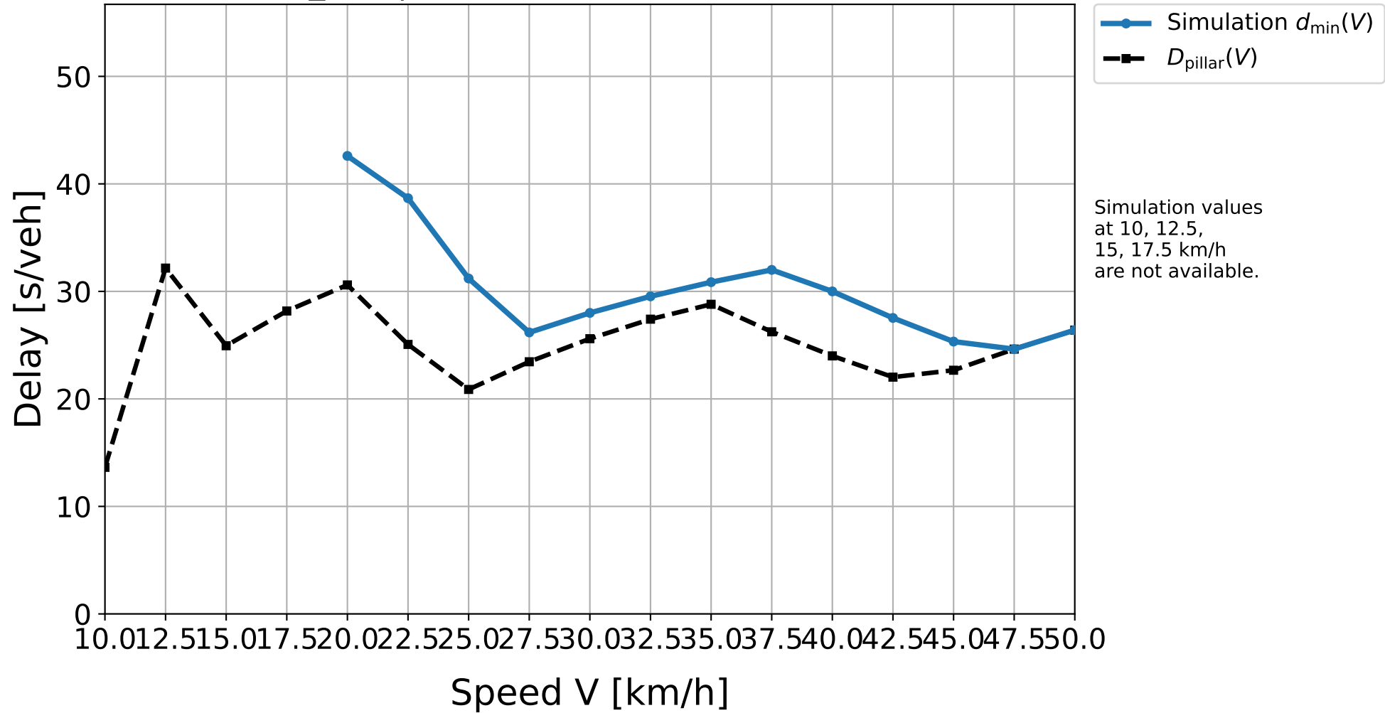
D10_323 | Simulation result vs. pillar delay
