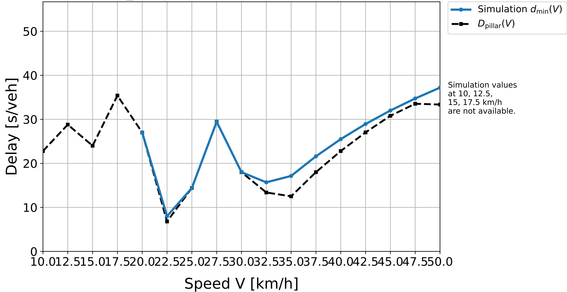
D30_333 | Simulation result vs. pillar delay
