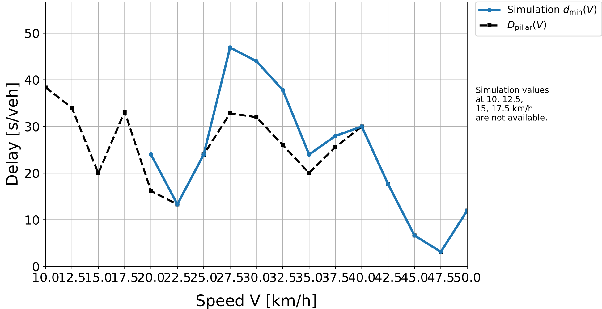
D50_323 | Simulation result vs. pillar delay
