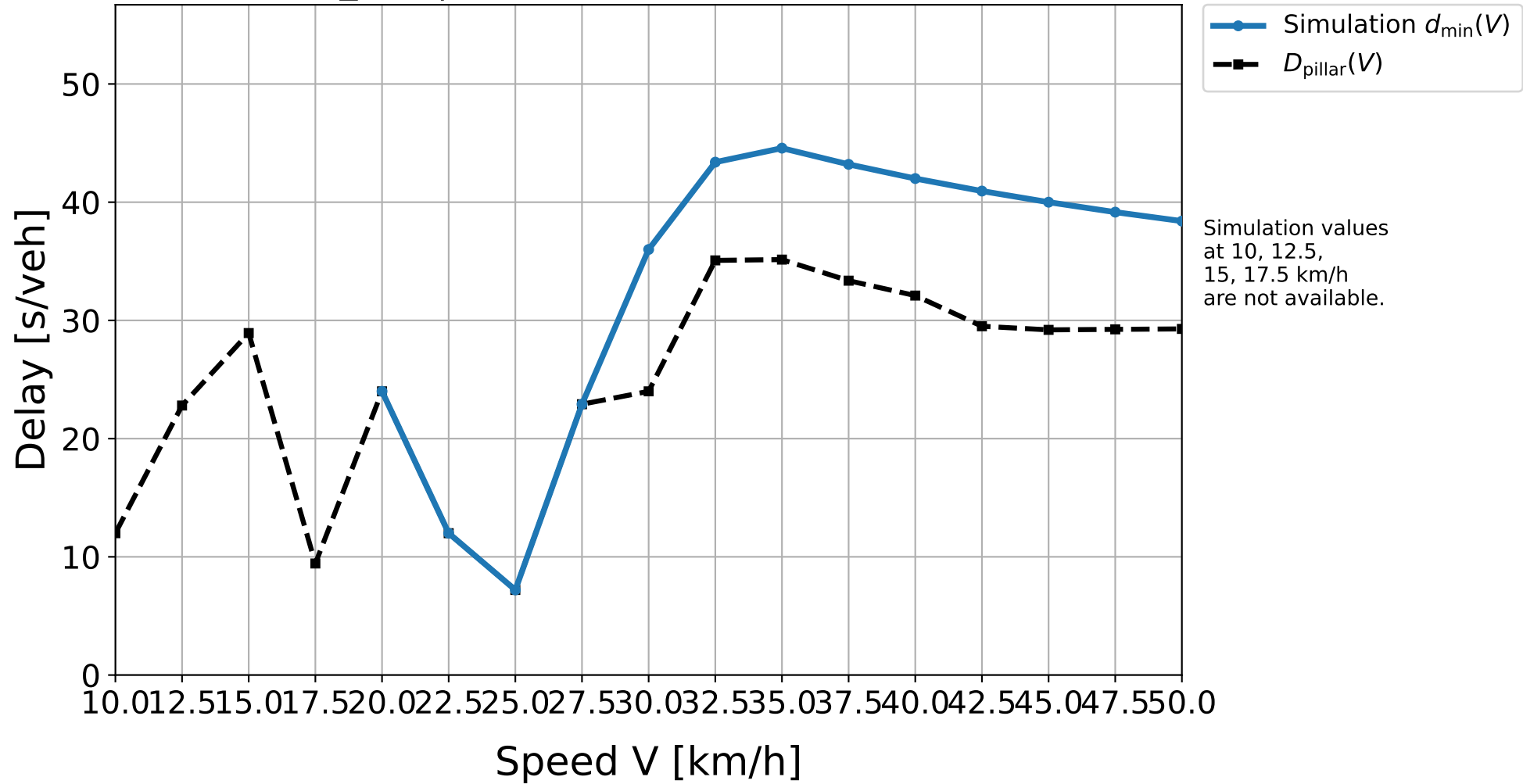
D30_322 | Simulation result vs. pillar delay
