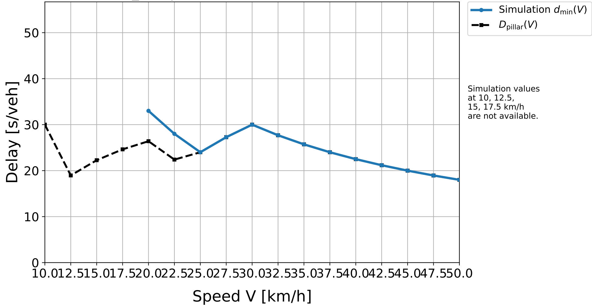
D10_331 | Simulation result vs. pillar delay
