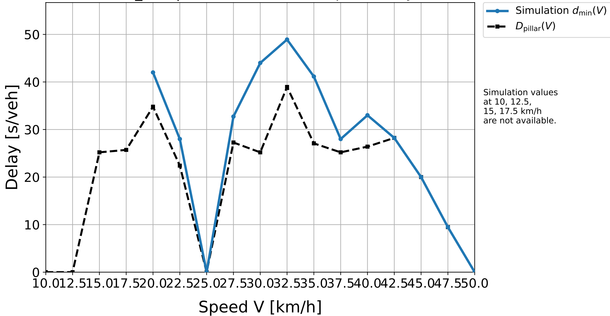
D50_H01 | Simulation result vs. pillar delay
