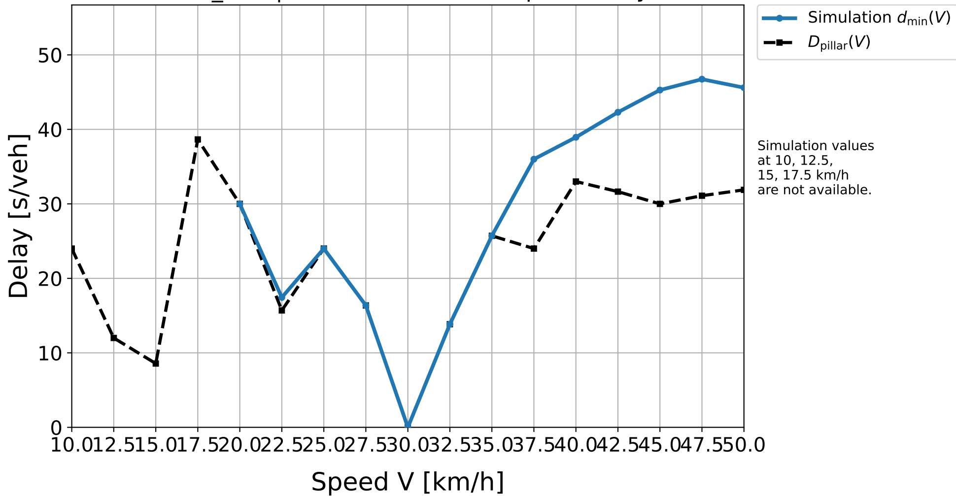
D30_H06 | Simulation result vs. pillar delay
